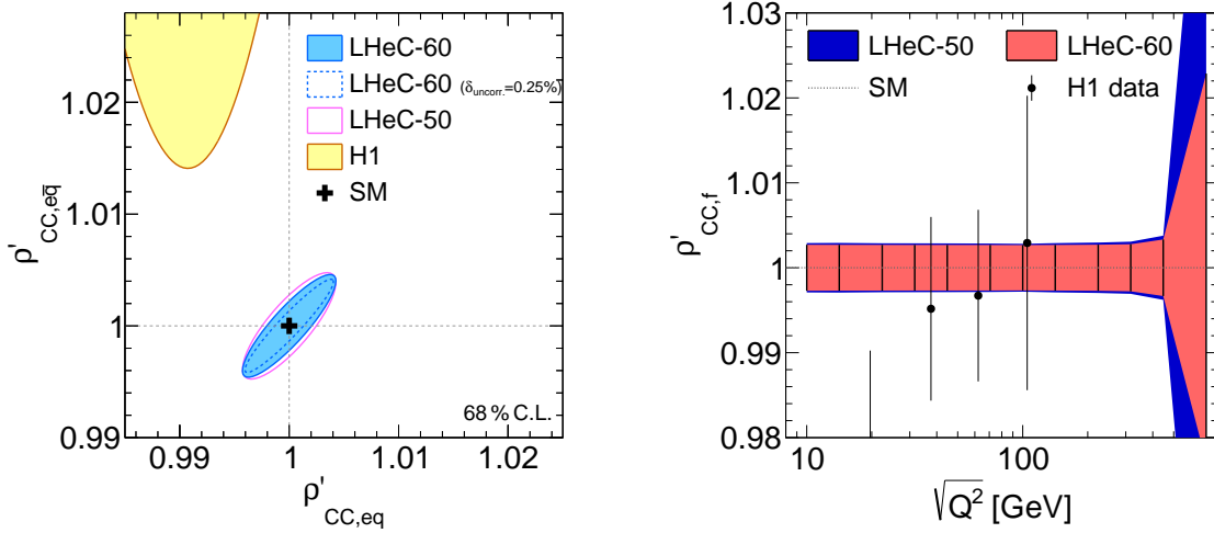
Figure 5.9: Left: anomalous modifications of the charged current form factors \rho'_{CC,eq} and \rho'_{CC,e\bar{q}} for different LHeC scenarios in comparison with the H1 measurement [415]. Right: scale dependent measurement of the anomalous modification of the charged current form factor \rho'_{CC}(Q^2) , assuming \rho'_{CC,eq} = \rho'_{CC,e\bar{q}} = \rho'_{CC} .
