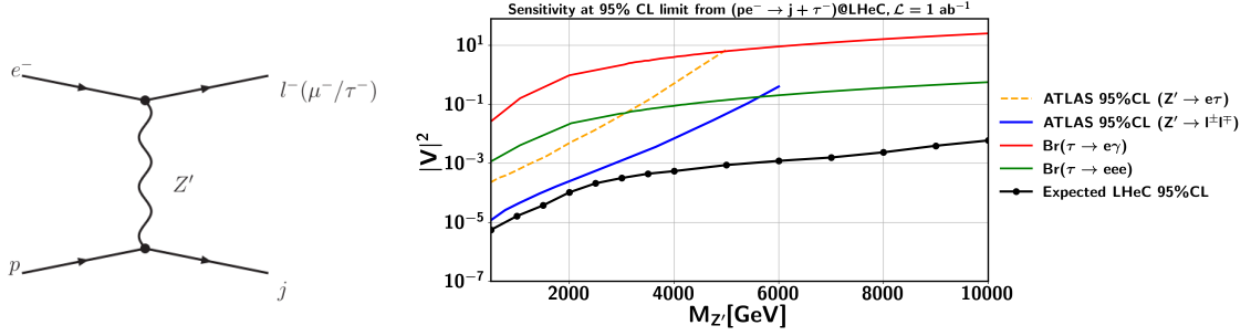
Figure 8.15: Left: Feynman diagram for the e - \tau (and e - \mu ) conversion processes pe^- \rightarrow \tau^- + j (and pe^- \rightarrow \mu^- + j ) mediated by a Z' with flavour-violating couplings to charged leptons at the LHeC. Right: Limits on the coupling parameter |V|^2 for signal hypothesis compared with the existing limits from experimental constraints on the relevant flavour conserving and flavour violating processes. The black line is the LHeC sensitivity for the process pe^- \rightarrow \tau j . For the other limits, see text.
