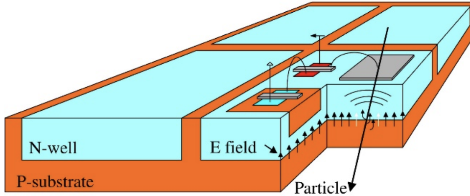
Figure 12.10: Typical sensor cross-section of a DMAPS detector in a HV-CMOS process [894].
