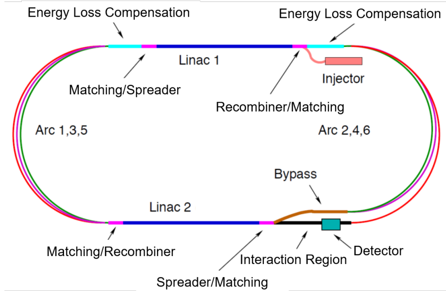
Figure 10.1: Schematic layout of the LHeC design based on an Energy Recovery Linac.
