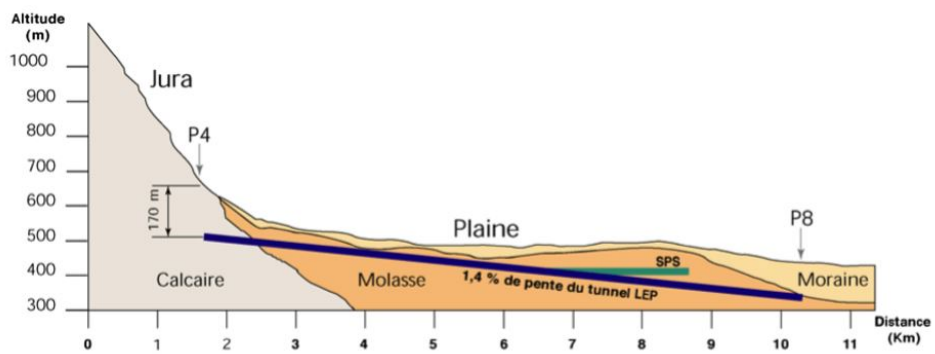
Figure 10.51: Geological profile of the LHC tunnel.
