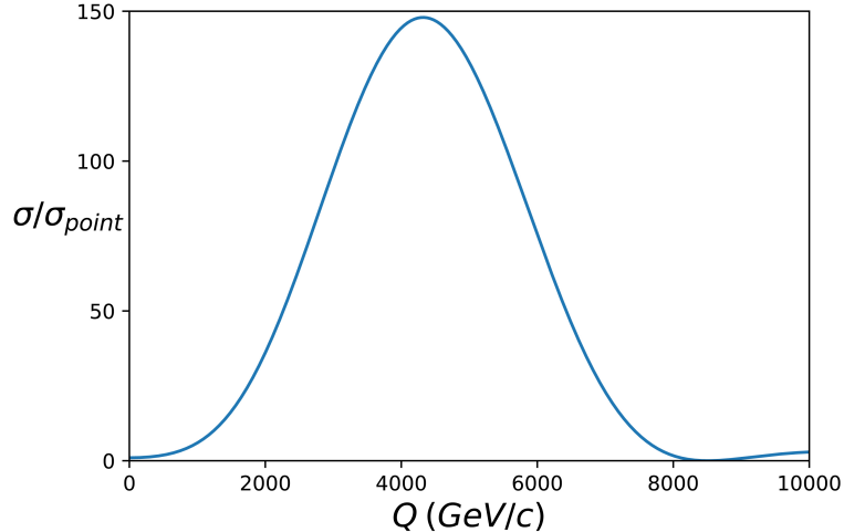
Figure 8.16: Form factor effect in the e-p interaction produced by substructure according to Model II of Hofstadter [700] with the model parameters given in the text.
