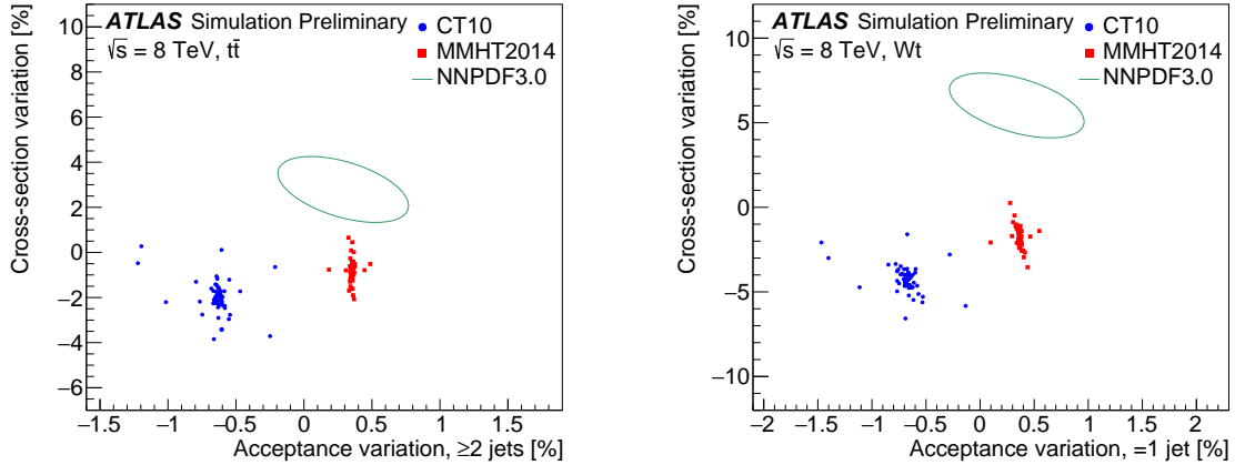
Figure 9.8: Impact of PDF uncertainty from CT10 and MMHT2014 eigenvectors or NNPDF3.0 replicas, on the cross section and the acceptance correction for top pair production t\bar{t} (left) and single top production Wt (right) (taken from Ref. [727]). Events are selected with at least two jets or with exactly one jet, respectively. Depending on the PDF set and eigenvector employed, the cross sections varies by up to 5–7% for top-pair and more than 10% for single-top production. Also the acceptance correction varies by about 0.5–1% for different PDF sets, and can become as large as 2.5% for different PDF sets and eigenvectors. Since the acceptance correction has to be imposed for the measurement, the limited knowledge of the PDFs introduces a sizeable modelling uncertainty on the measurement.
