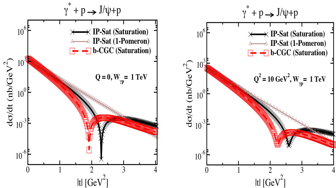
Figure 3.23: Differential cross section for the elastic J/\psi production as a function of |t| within the IP-Sat (saturation), b-CGC and 1-Pomeron models at a fixed W_{\gamma p} = 1 \text{ TeV} , which corresponds to the LHeC kinematics, and for two different values of photon virtuality Q = 0 and Q^2 = 10 \text{ GeV}^2 . The thickness of points includes the uncertainties associated with the freedom to choose different values for the charm quark mass within the range m_c = 1.2 - 1.4 \text{ GeV} .
