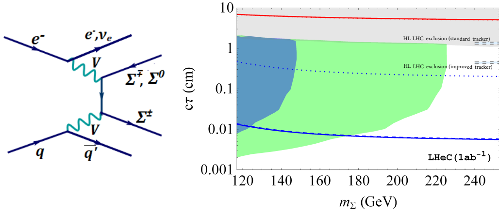
Figure 8.9: Left: Dominant production diagram of triplet fermion pairs via their gauge interactions. Right: Prospects of displaced vertex searches from charged fermion triplet \Sigma^{\pm} . The blue and green shaded regions denote the expected observability of 10 (100) events, dashed lines denote HL-LHC exclusion sensitivity, and the red line is connected to the light neutrino properties. For details, see text and Ref. [659].
