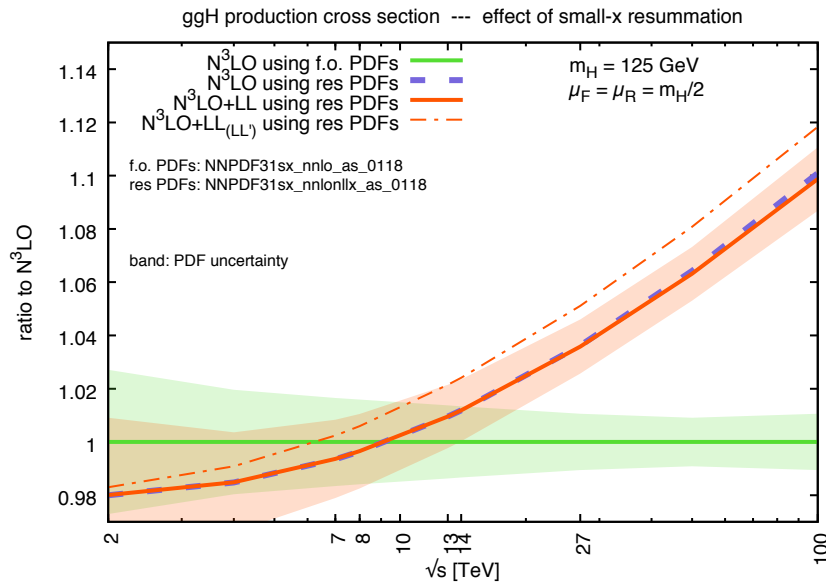
Figure 9.13: Ratio of the N 3 LO Higgs cross section with and without resummation to the N 3 LO fixed-order cross section, as a function of the collider centre-of-mass energy. “f.o.” denotes fixed order, “res” denotes resummed and “LL” a different anomalous dimension matching at leading logarithmic accuracy, see the legend on the plot and Ref. [758] for details. The PDFs used are from the global dataset of Ref. [250]. Figure taken from Ref. [758].
