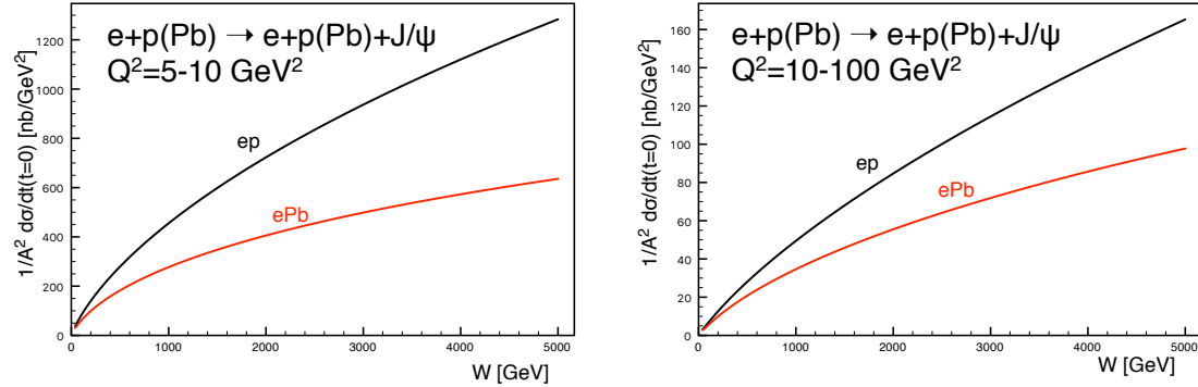
Figure 6.13: Cross section for the coherent diffractive production of the vector meson J/\psi in ePb (red solid curves) and ep (black solid curves) collisions, as a function of the energy W . Left: Q^2 = 5 - 10 \text{ GeV}^2 , right: Q^2 = 10 - 100 \text{ GeV}^2 .
