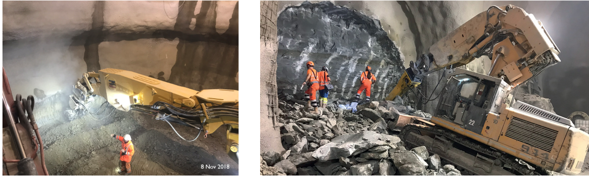
Figure 10.54: Left: Roadheader being used for shaft excavation at HL-LHC Point 1. Right: Rockbreaker used for new service tunnels excavation at HL-LHC Point 5 (Credit: Z. Arenas).
