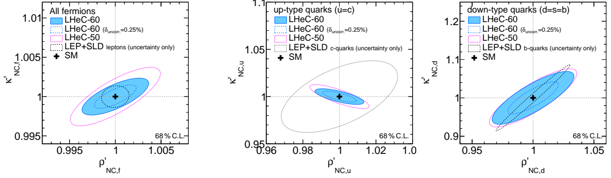
Figure 5.5: Expectations at 68 % confidence level for the determination of the \rho'_{\text{NC}} and \kappa'_{\text{NC}} parameters assuming a single anomalous factor equal for all fermions (left). The results for three different LHeC scenarios are compared with the achieved uncertainties from the LEP+SLD combination [436] for the determination the respective leptonic quantities. Right: uncertainties for the simultaneous determination of the anomalous form factors for u and d -type quarks, assuming known values for the electron parameters. The values are compared with uncertainties reported by LEP+SLD for the determination of the values \rho_{\text{NC},(c,b)} and \sin\theta_{\text{W}}^{\text{eff},(c,b)} for charm or bottom quarks, respectively.
