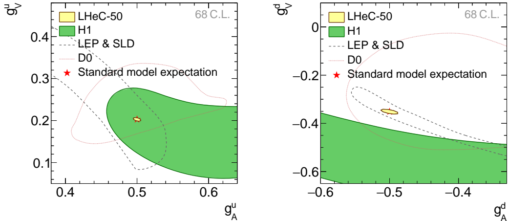
Figure 5.4: Weak NC vector and axial-vector couplings of u -type (left) and d -type quarks (right) at 68 % confidence level (C.L.) for simulated LHeC data with E_e = 50 GeV. The LHeC expectation is compared with results from the combined LEP+SLD experiments [436], a single measurement from D0 [437] and one from H1 [415]. The standard model expectations are displayed by a red star, partially hidden by the LHeC prospects.
