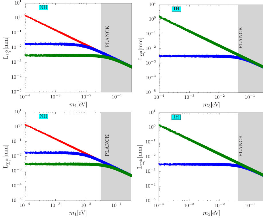
Figure 8.8: Proper decay length of \Sigma_i^0(\Sigma_i^\pm) with respect to the lightest light neutrino mass in the upper (lower) panel for 1 TeV triplet. The Normal (Inverted) hierarchy case is shown in the left (right) panel. The first generation triplet is represented by the red band, the second generation is represented by the blue band and the third generation is represented by the green band respectively. The shaded region is excluded by the PLANCK data [658].
