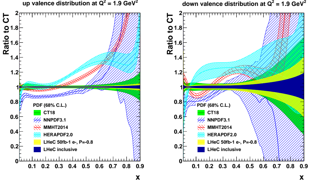
Figure 3.8: Valence quark distributions at Q^2 = 1.9 \text{ GeV}^2 as a function of x , presented as the ratio to the CT18 [66] central values. The yellow band corresponds to the “LHeC 1st run” PDFs (D2), while the dark blue shows the final “LHeC inclusive” PDFs based on the data sets (D4+D5+D6+D9), as described in Sect. 3.3.1. For the purposes of illustrating the improvement to the uncertainties more clearly, the central values of the LHeC PDFs have been scaled to the CT18 PDF, which itself is displayed by the green band.
