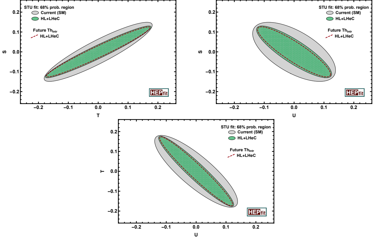
Figure 9.4: Allowed regions in the (S, T, U) plane showing all three combinations: S vs T (top-left), S vs U (top-right), T vs U (bottom). The grey and green areas indicate the currently allowed region and the LHeC projection, respectively. The dashed line indicates the effect of expected theoretical improvements. The HEPfit program [719] was used for this analysis.
