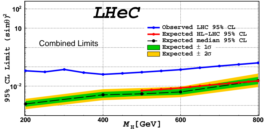
Figure 8.2: Expected exclusion limits (green and yellow bnds) for a heavy scalar search at the LHeC, assuming a systematic uncertainty on the SM background of 2% (from Ref. [627]). The blue line represents the current LHC limit at 95% CL as extracted from [628], the red line the forecast of the HL-LHC sensitivity via h_2 \rightarrow ZZ searches from Ref. [629]. The LHeC results correspond to an integrated luminosity of 1 \text{ ab}^{-1} .
