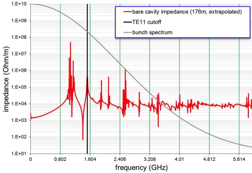
Figure 4.14: Dipole HOM spectrum of the bare cavity. All harmful modes are well separated from RF harmonics. Impedances of modes below cut-off are unresolved and will be determined by the HOM damping configuration.
