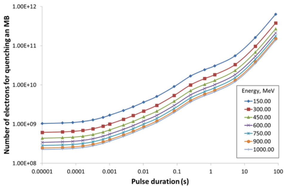
Figure 2.3: Amount of impacting particles versus pulse length to reach the quench level of a LHC main dipole. The energy density distribution is taken from the FLUKA simulations shown in Fig. 2.1 and 2.2.
