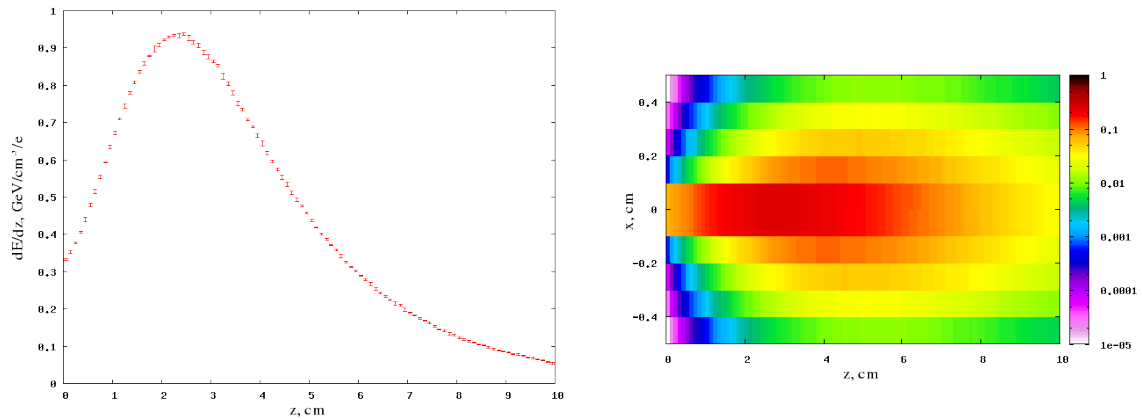
Figure 2.2: Maximum values of energy deposition (left) and projection of energy deposition (right) for 1 GeV electrons impacting in a solid copper block as calculated by FLUKA [17, 18]. An emittance of 50 \mu\text{m} and a beta-function at extraction of 5 m was used. The bin size was 1 \text{ mm}^3 .
