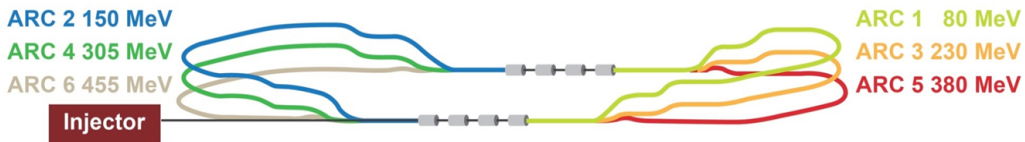
Figure 3.3: A second phase with recirculation could feature three-pass operation to reach 455 MeV.
