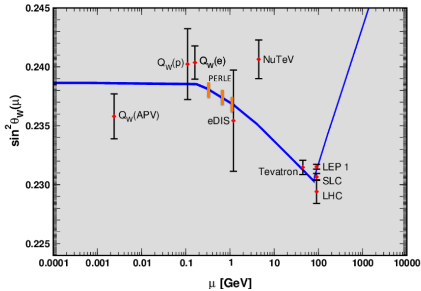
Figure 2.4: Prospect for the measurement of the weak mixing angle with PERLE (illustration of half a percent accuracy measurement) based on the polarisation asymmetry A^- , as compared to the current status of \sin^2 \theta_W measurements, from PDG2014.
