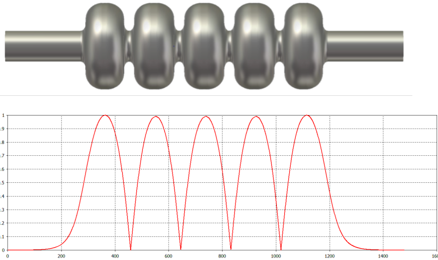
Figure 4.8: Cavity design (single-die, iris ID=tube ID) 801.58 MHz (top); Axial field on axis (bottom).
