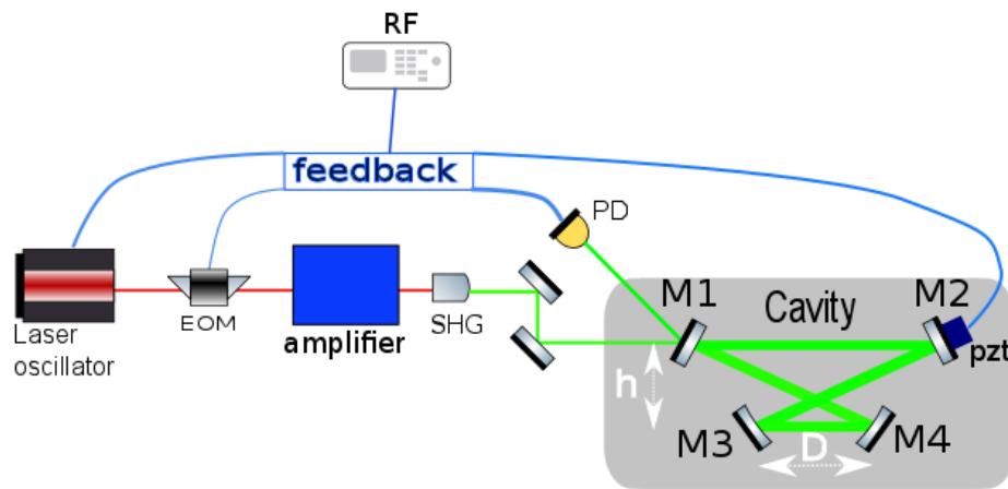
Figure 4.30: Simplified scheme of a four mirror cavity locked to an amplified laser oscillator. Planar ( M_1 and M_2 ) and concave ( M_3 and M_4 ) mirrors are shown along with the electro-optic modulator (EOM) used to build the feedback error signal from the reflected signal (photodiode PD) and a piezo-electric transducer (PZT) fixed on M_2 to synchronize the cavity round trip frequency to the accelerator RF.
