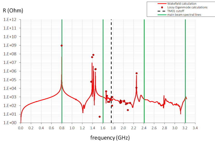
Figure 4.9: Impedance spectrum for the longitudinal modes as a function of frequency of the low-loss cavity design with iris diameter of 130 mm (compare Fig. 4.4).
