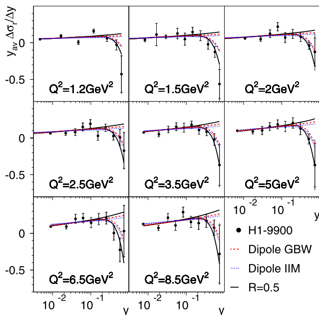
Fig. 35 Derivative y_{\text{av}} \Delta\sigma / \Delta y for the combined 1999–2000 H1 data compared to the predictions of the dipole models and the fractal model for F_2 with an assumption R = 0.5 to describe F_L , labeled R = 0.5 . The lines increasing as a function of \ln y correspond to F_L = 0 for these models. The lines turning over at high y correspond to the cross section predictions. The inner error bars represent statistical and uncorrelated uncertainties added in quadrature, the outer error bars represent the total uncertainties
