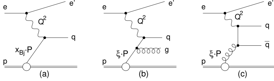
Figure 3.20: Leading order diagrams for inclusive DIS (a) and jet production (b,c) in the Breit frame (taken from Ref. [86]).
