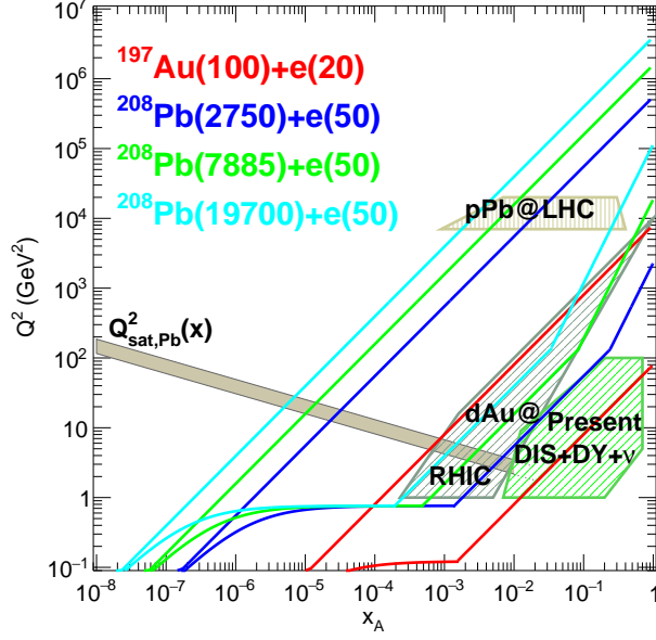
Figure 4.1: Kinematic regions in the x - Q^2 plane explored by different data sets (charged lepton and neutrino DIS, DY, dAu at RHIC and pPb at the LHC) used in present nPDF analyses [405], compared to the ones achievable at the EIC (red), the LHeC (ERL against the HL-LHC beams, dark blue) and two FCC-eh versions (with Pb beams corresponding to proton energies E_p = 20 TeV - green and E_p = 50 TeV - light blue). Acceptance of the detector for the electrons is taken to be 1^\circ < \theta < 179^\circ , and 0.01(0.001) < y < 1 for the EIC (all other colliders). The saturation scale Q_{sat} shown here for indicative purposes only, see also [406], has been drawn for a Pb nucleus considering an uncertainty \sim 2 and a behaviour with energy following the model in [407]. Note that it only indicates a region where saturation effects are expected to be important but there is no sharp transition between the linear and non-linear regimes.
