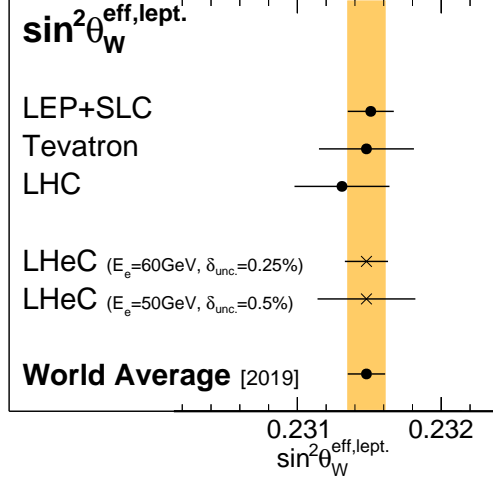
Figure 3.56: Comparison of the determination of \sin^2 \theta_W^{\text{eff},\ell}(M_Z^2) from LHeC inclusive DIS data with recent averaged values. Results from LEP+SLC [340], Tevatron [342], LHC [343–346] and the world average value [346] are all obtained from a combination of various separate measurements (not shown individually) (see also Ref. [347] for additional discussion). For LHeC, the experimental and PDF uncertainties are displayed.
