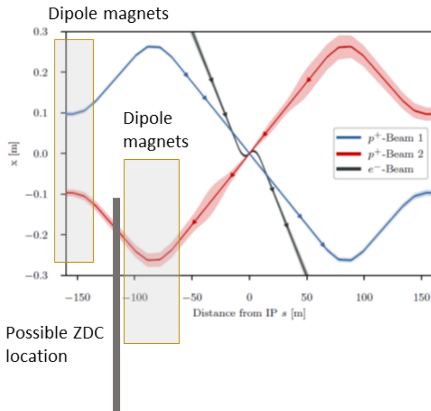
Figure 10.10: Possible location of a ZDC for the linac–ring design of LHeC. The solid rectangle represents the ZDC. The two boxes in front of and behind the ZDC indicate the locations for bending magnets.
