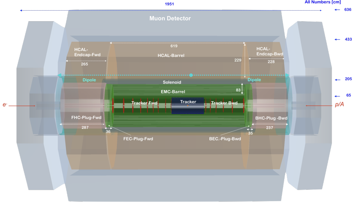
Figure 10.11: Side view of a lowE-FCCeh ( E_p = 20\text{TeV} ) concept detector designed using the DD4hep framework [ref.] showing essential measures. The principal layout is similar to the LHeC detector. As well as the choice of materials (warm version). The experiment solenoid is placed again between the ECAL-Barrel and Hadronic-Barrel calorimeter (HCAL-Barrel) and housed in a cryostat common with the beam steering dipoles extending over the full length of the HCAL-Barrel and HCAL-Plug-forward/backward. The sizes has been chosen such that the solenoid/dipoles and ECAL-Barrel systems as well as the whole tracker serve also after an upgrade of beam energy to E_p = 50\text{TeV} and an upgrade of detector accordingly.
