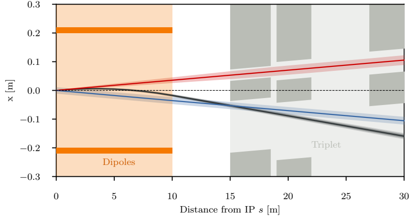
Figure 8.30: Empty space between the detector dipole and the superconducting quadrupoles of the final focus triplet.
