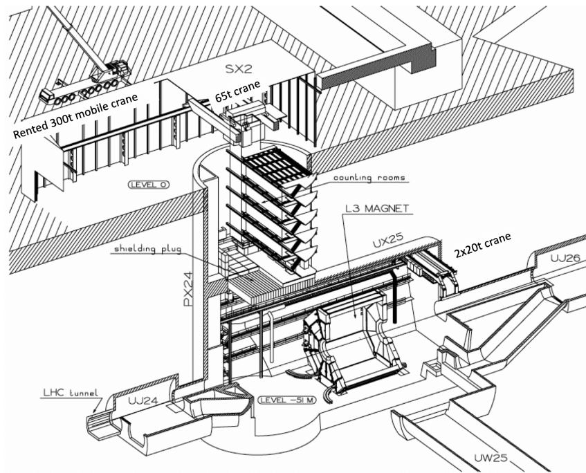
Figure 10.13: View on the cavern infrastructure at Point 2. In the centre one recognises the support structure of the magnet of the L3 experiment which is thought to house and support also the LHeC detector, not least for its removal would cost significant extra time.
