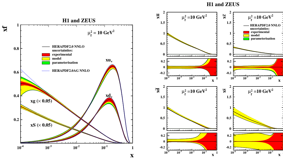
Figure 3.4: Left: HERAPDF2.0NNLO PDFs for valence, gluon and total Sea, showing experimental, model and parametrisation uncertainties separately, at factorisation scale \mu_f = 10\text{GeV}^2 . An alternative (AG) PDF with no negative term added to the gluon parametrisation is also shown. Right: HERAPDF2.0NNLO PDFs for the Sea, x\bar{u}, x\bar{d}, x\bar{c}, x\bar{s} showing experimental, model and parametrisation uncertainties separately, at factorisation scale \mu_f = 10\text{GeV}^2 . Fractional uncertainties are shown below the plots
