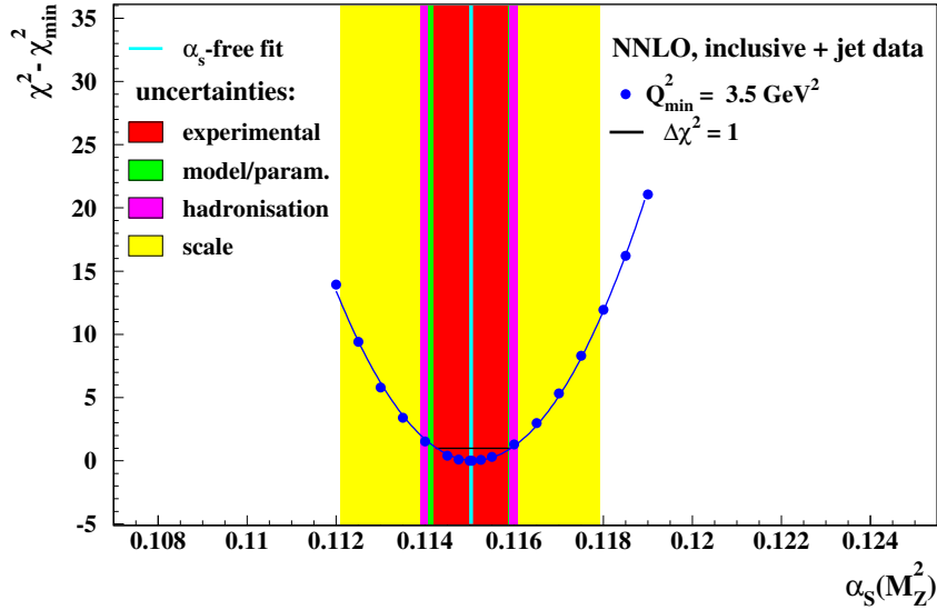
Figure 3.6: \Delta\chi^2 = \chi^2 - \chi_{min}^2 vs. \alpha_S(M_Z) for HERAPDF2.0Jets NNLO (prel.) fits with fixed \alpha_S(M_Z) .
