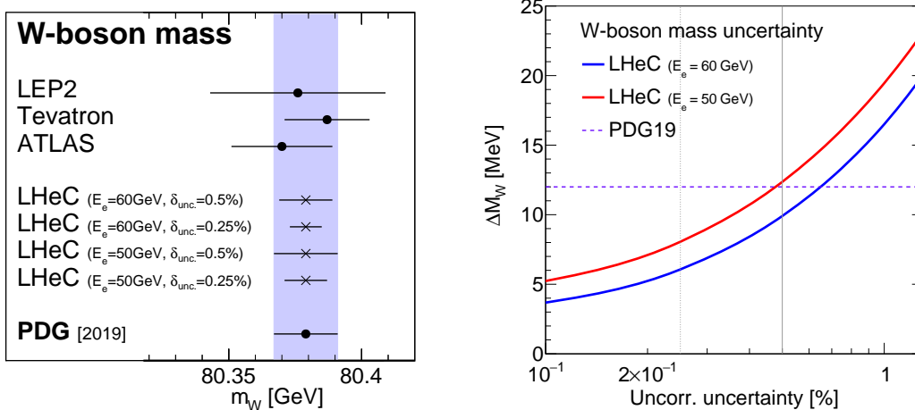
Figure 3.51: Left: Measurements of the W -boson mass assuming fixed values for the top-quark and Z -boson masses at the LHeC for different scenarios in comparison with today’s measurements [333–335] and the world average value (PDG19) [133]. For LHeC, prospects for E_e = 60 GeV and 50 GeV are displayed, as well as results for the two scenarios with 0.5 % or 0.25 % uncorrelated uncertainty (see text). Right: Comparison of the precision for M_W for different assumptions of the uncorrelated uncertainty of the pseudo-data. The uncertainty of the world average value is displayed as horizontal line. The nominal (and alternative) size of the uncorrelated uncertainty of the inclusive NC/CC DIS pseudo-data is indicated by the vertical line (see text).
