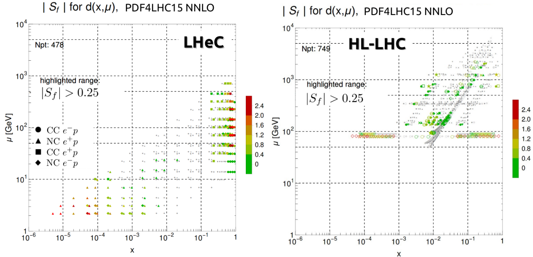
Figure 3.3: Sensitivity for a sample flavor \{d(x, Q)\} in the \{x, Q^2\} kinematic plane for the LHeC (left) and the HL-LHC (right) calculated with pseudodata [40]. We observe the LHeC is particularly sensitive in both the high and low x regions, and the HL-LHC covers the intermediate x region out to large Q scales.
