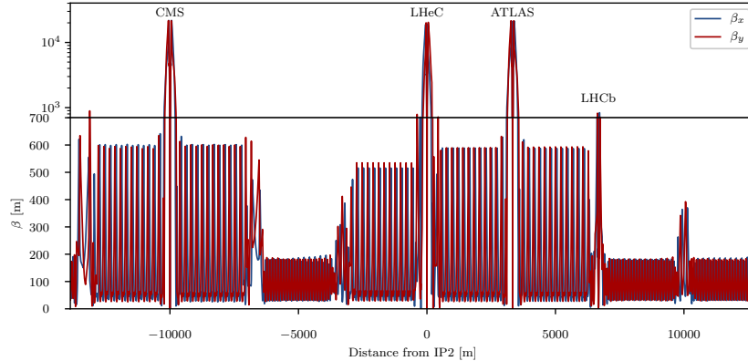
Figure 8.28: Optics of full ring of the colliding LHC proton beam (Beam 2).
