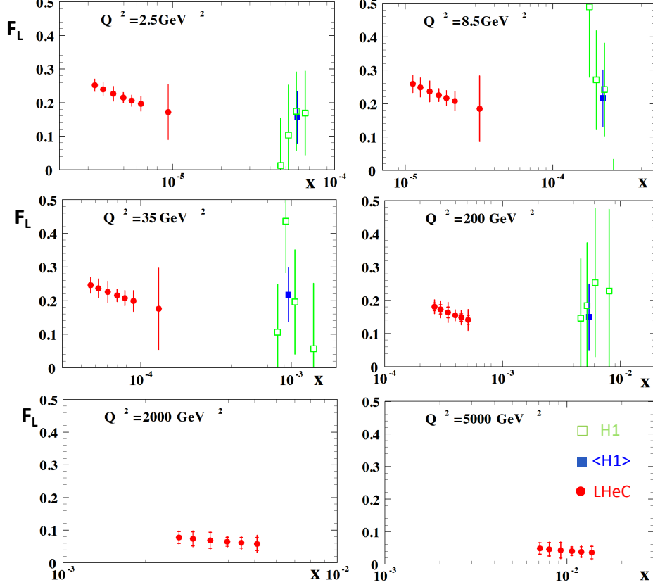
Figure 3.33: H1 measurement and LHeC simulation of data on the longitudinal structure function F_L(x, Q^2) . Green: Data by H1, for selected Q^2 intervals from Ref. [210]; Blue: Weighted average of the (green) data points at fixed Q^2 ; Red: Simulated data from an F_L measurement at the LHeC with varying beam energy, see text. The H1 error bars denote the total measurement uncertainty. The LHeC inner error bars represent the data statistics, visible only for Q^2 \geq 200 \text{ GeV}^2 , while the outer error bars are the total uncertainty. Since the F_L measurement is sensitive only at high values of inelasticity, y = Q^2/sx , each Q^2 value is sensitive only to a certain limited interval of x values which increase with Q^2 . Thus each diagram has a different x axis. The covered x range similarly varies with s , i.e. H1 x values are roughly twenty times larger at a given Q^2 . There are no H1 data for high Q^2 , beyond 1000 \text{ GeV}^2 , see Ref. [210].
