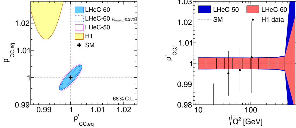
Figure 3.57: Left: anomalous modifications of the charged current form factors \rho'_{CC,eq} and \rho'_{CC,e\bar{q}} for different LHeC scenarios in comparison with the H1 measurement [318]. Right: scale dependent measurement of the anomalous modification of the charged current form factor \rho'_{CC}(Q^2) , assuming \rho'_{CC,eq} = \rho'_{CC,e\bar{q}} = \rho'_{CC} .
