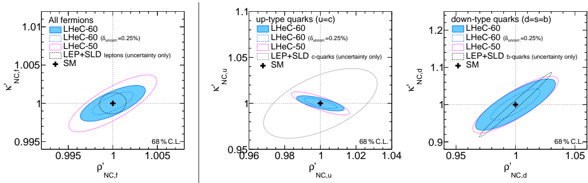
Figure 3.54: Expectations at 68 % confidence level for the determination of the \rho'_{\text{NC}} and \kappa'_{\text{NC}} parameters assuming a single anomalous factor equal for all fermions (left). The results for three different LHeC scenarios are compared with the achieved uncertainties from the LEP+SLD combination [340] for the determination the respective leptonic quantities. Right: uncertainties for the simultaneous determination of the anomalous form factors for u and d -type quarks, assuming known values for the electron parameters. The values are compared with uncertainties reported by LEP+SLD for the determination of the values \rho_{\text{NC},(c,b)} and \sin\theta_{\text{W}}^{\text{eff},(c,b)} for charm or bottom quarks, respectively.
