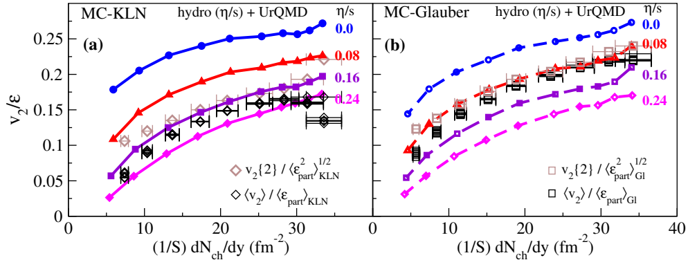
Figure 7.3: Comparison of the universal v_2(\eta/s)/\epsilon vs. (1/S)(dN_{ch}/dy) curves with experimental data for \langle v_2 \rangle [567], v_2\{2\} [568], and dN_{ch}/dy [569] from the STAR Collaboration. The experimental data used in (a) and (b) are identical, but the normalisation factors \langle \epsilon_{part} \rangle and S used on the vertical and horizontal axes, as well as the factor \langle \epsilon_{part}^2 \rangle^{1/2} used to normalize the v_2\{2\} data, are taken from the MC-KLN model in (a) and from the MC-Glauber model in (b). Theoretical curves are from simulations with MC-KLN initial conditions in (a) and with MC-Glauber initial conditions in (b). Taken from [563].
