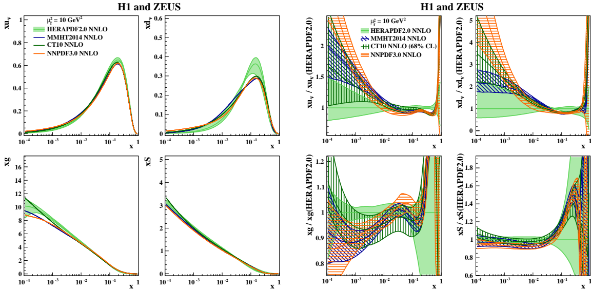
Figure 3.5: The HERAPDF2.0NNLO PDFs for valence, gluon and total Sea compared to other NNLO PDF sets MMHT14, CT10, NNPDF3.0, at factorisation scale \mu_f = 10\text{GeV}^2 . Left; PDFs: right; ratios of PDFs to the HERAPDF. Total uncertainties are shown for the HERAPDFs in both the left and right hand side plots, whereas total uncertainties for the MMHT,CT and NNPDF PDFs are only shown on the right hand side plots.
