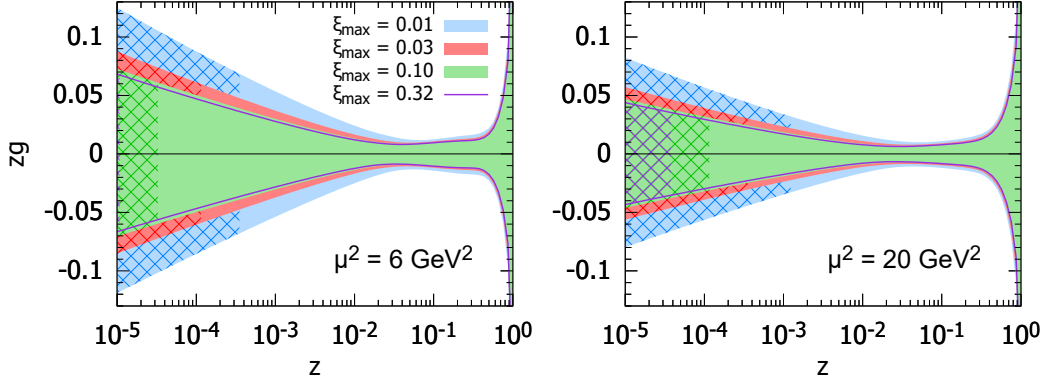
Figure 3.42: Relative uncertainties on the diffractive gluon PDFs for the LHeC kinematics. Two different choices of scales are considered \mu^2 = 6 and \mu^2 = 20 \text{ GeV}^2 . The blue, red, green bands and magenta line correspond to different maximal values of \xi = 0.01, 0.03, 0.1, 0.32 , respectively. The cross-hatched areas show kinematically excluded regions. The bands indicate only the experimental uncertainties, see the text.
