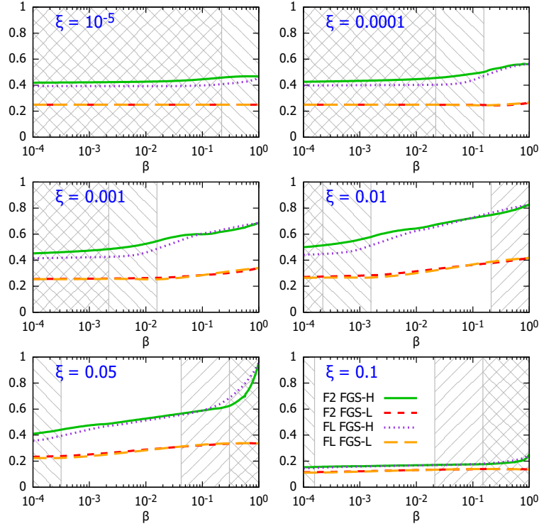
Figure 4.16: Nuclear modification factor, Eq. (4.10), for F_2^{D(3)} and F_L^{D(3)} in ^{208}\text{Pb} versus \beta , at Q^2 = 10 \text{ GeV}^2 and for different \xi , for the models H and L in [408]. The ‘\’ and ‘/’ hatched areas show kinematically excluded regions for E = 2.76 and 19.7 \text{ TeV/nucleon} , respectively.
