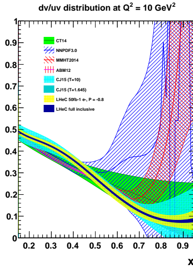
Figure 3.11: The d_v/u_v distribution at Q^2 = 10 \text{ GeV}^2 as a function of Bjorken x . The yellow band corresponds to the “LHeC 1st run” PDFs ( D2 ), while the dark blue shows the “LHeC full inclusive” PDFs ( D4+D5+D7+D8 ), as described in the text. Both LHeC PDFs shown are scaled to the central value of CT14.
