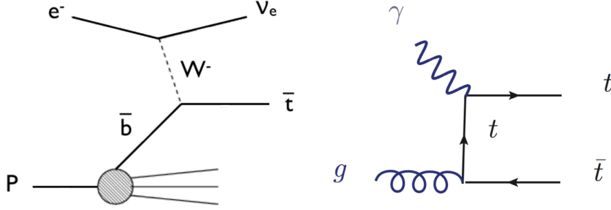
Figure 3.60: Example graphs for CC DIS top quark production (left) and top quark photoproduction (right).
