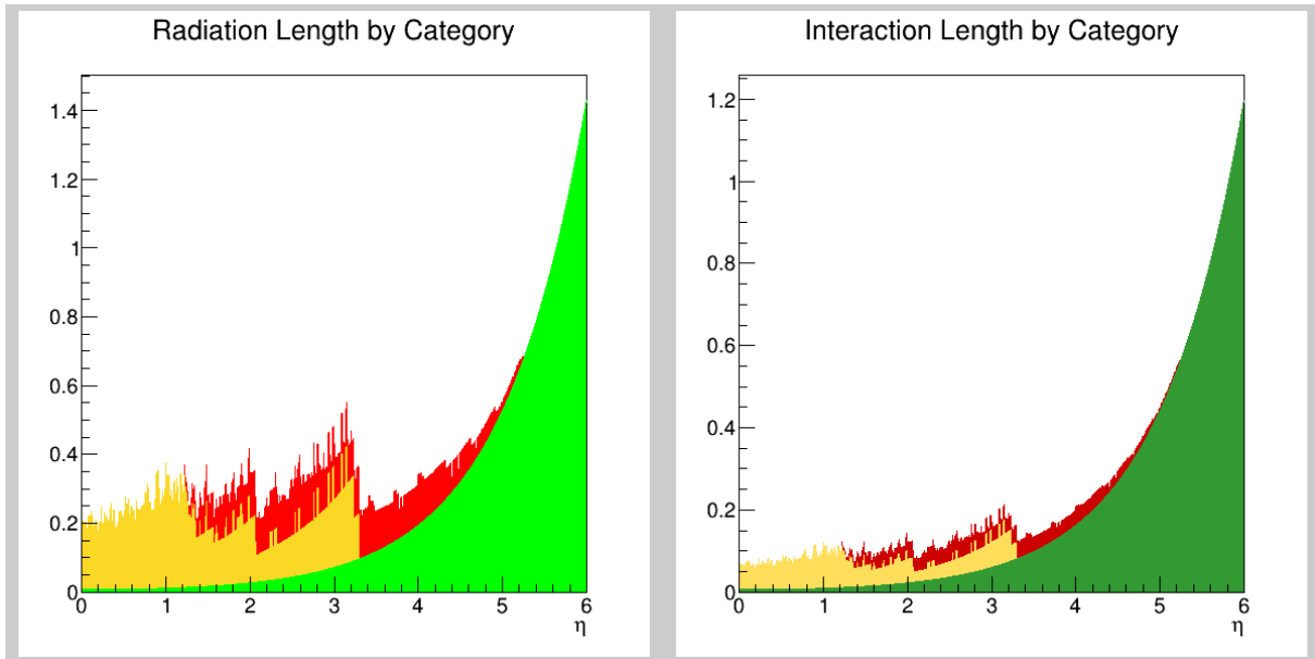
Figure 10.9: Material contributions from the tracking modules as a function of pseudorapidity. Results are given in terms of radiation lengths (left) and hadronic interaction lengths (right). The results are broken down into contributions from barrel modules (yellow) and endcap / additional disk modules (red) and are compared with the contribution from the 2.5 mm beam pipe (green).
