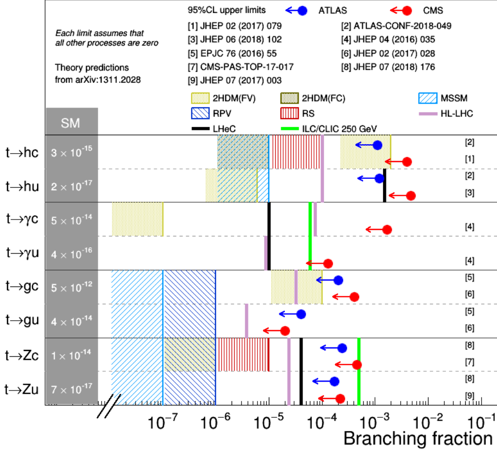
Figure 3.62: Comparison of top quark FCNC branching ratio limits at the LHC, HL-LHC, LHeC, and ILC/CLIC colliders.
