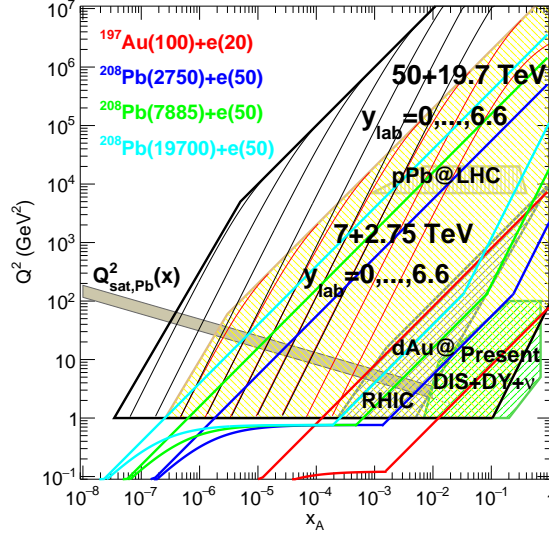
Figure 7.4: Kinematic regions in the x - Q^2 plane explored by data sets (charged lepton and neutrino DIS, DY, dAu at RHIC and pPb at the LHC) used in present nPDF analyses [405], compared to the ones achievable at the EIC (red), the LHeC (ERL against the HL-LHC beams, dark blue) and two FCC-eh versions (with Pb beams corresponding to proton energies of 20 TeV - green and 50 TeV - light blue). Acceptance is taken to be 1^\circ < \theta < 179^\circ , and 0.01(0.001) < y < 1 for the EIC (all other colliders). The areas delimited by thick brown and black lines show the regions accessible in pPb collisions at the LHC and the FCC-hh (50 TeV) respectively, while the thin lines represent constant rapidities from 0 (right) to 6.6 (left) for each case. The saturation scale Q_{sat} shown here for indicative purposes only, see also [406], has been drawn for a Pb nucleus considering an uncertainty \sim 2 and a behaviour with energy following the model in [407]. Note that it only indicates a region where saturation effects are expected to be important but there is no sharp transition between the linear and non-linear regimes.
