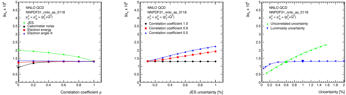
Figure 3.22: Studies of the size and correlations of experimental uncertainties impacting the uncertainty of \alpha_s(M_Z) . Left: Study of the value of the correlation coefficient \rho for different systematic uncertainties. Common systematic uncertainties are considered as fully correlated, \rho = 1 . Middle: Size of the JES uncertainty for three different values of \rho_{\text{JES}} . Right: Impact of the uncorrelated and normalisation uncertainties on \Delta\alpha_s(M_Z) .
