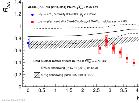
Figure 7.2: ALICE inclusive J/\psi nuclear modification factor versus rapidity [562], compared to nPDF calculations. Taken from [559].
