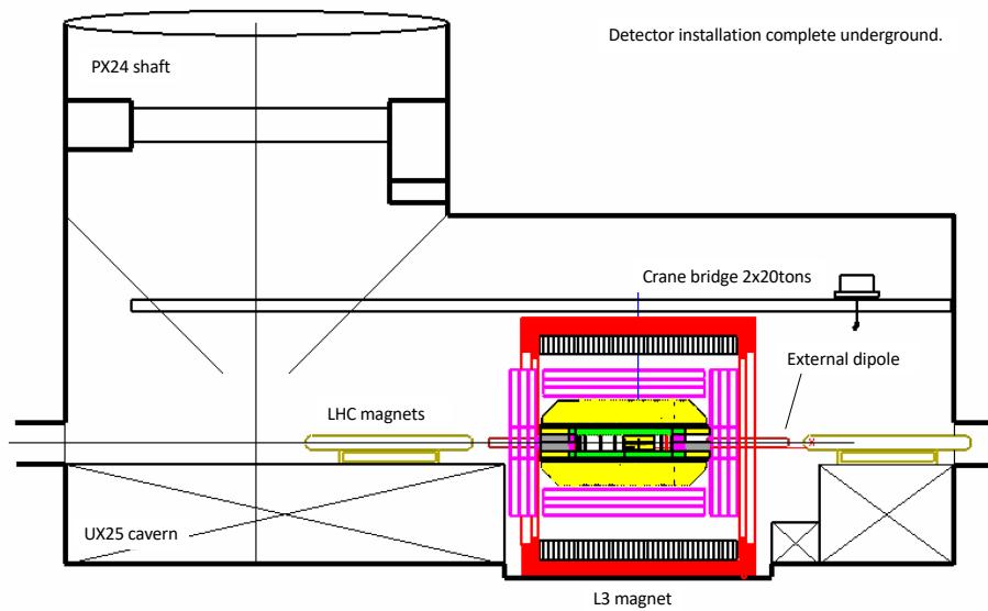
Figure 10.14: View on the LHeC detector, housed in the L3 magnet support structure, after installation at the interaction point.
