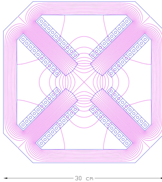
Figure 8.14: ERL - Cross section of the linac quadrupole magnets.
