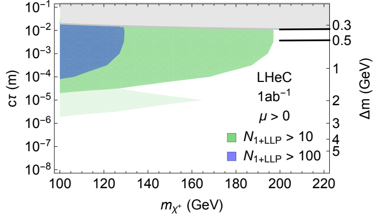
Figure 6.4: Exclusion limits on Higgsino masses as a function of their lifetime from Ref. [496]. Coloured regions denote where 10 or 100 events with at least one LLP decay are observed. Light shading indicates the uncertainty in the predicted number of events due to different hadronisation and LLP reconstruction assumptions. The black curves are the optimistic and pessimistic projected bounds from HL-LHC disappearing track searches.
