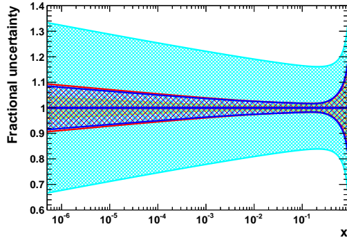
(c) \bar{d} quark distribution.
