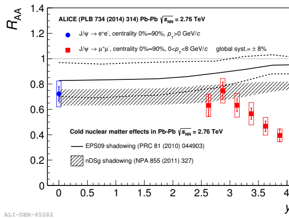
Figure 7.8: ALICE inclusive J/\psi nuclear modification factor versus rapidity [570], compared to nPDF calculations. Taken from [567].
