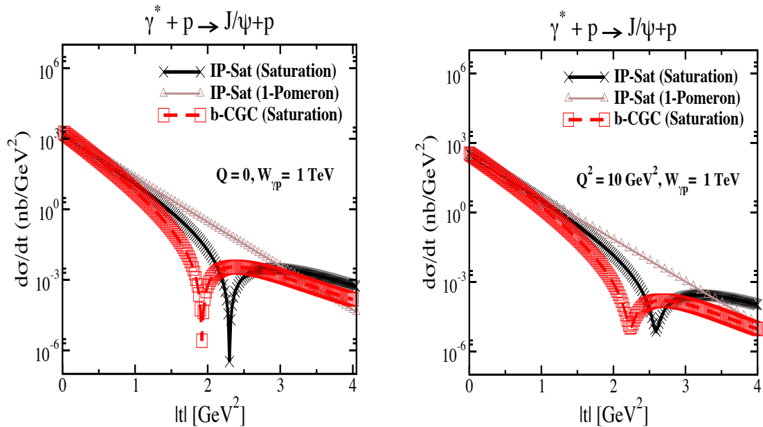
Figure 3.35: Differential cross section for the elastic J/\psi production as a function of |t| within the IP-Sat (saturation), b-CGC and 1-Pomeron models at a fixed W_{\gamma p} = 1 \text{ TeV} , which corresponds to the LHeC kinematics, and for two different values of photon virtuality Q = 0 and Q^2 = 10 \text{ GeV}^2 . The thickness of points includes the uncertainties associated with the freedom to choose different values for the charm quark mass within the range m_c = 1.2 - 1.4 \text{ GeV} .
