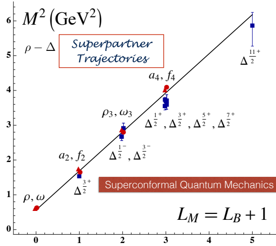
Figure 3.45: Comparison of the \rho/\omega meson Regge trajectory with the J = 3/2 \Delta baryon trajectory. Superconformal algebra predicts the mass degeneracy of the meson and baryon trajectories if one identifies a meson with internal orbital angular momentum L_M with its superpartner baryon with L_M = L_B + 1 . See Refs. [294, 297].
