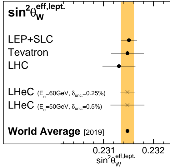
Figure 3.56: Comparison of the determination of \sin^2 \theta_{\text{W}}^{\text{eff},\ell}(M_Z^2) from LHeC inclusive DIS data with recent averaged values. Results from LEP+SLC [338], Tevatron [340], LHC [341–344] and the world average value [344] are all obtained from a combination of various separate measurements (not shown individually) (see also Ref. [345] for additional discussions). For LHeC, the experimental and PDF uncertainties are displayed.
