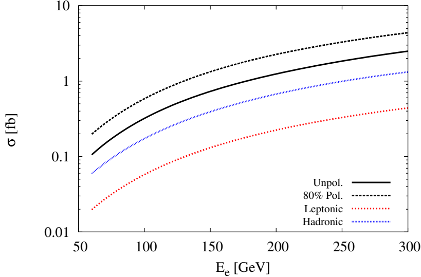
Figure 5.3: Cross-sections of the Higgs boson produced in association with a top quark in e^-p collisions with E_p = 7 TeV. for different electron beam energies. The dotted and solid black lines correspond to p e^- \rightarrow \bar{t} h \nu_e with and without longitudinal polarisation of the electron beam, respectively. The dotted red and blue lines correspond to \sigma \times \text{BR} for the leptonic and hadronic decay modes of \bar{t} where for this estimation we use basic cuts (see text).
