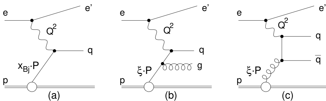
Figure 3.20: Leading order diagrams for inclusive DIS (a) and jet production (b,c) in the Breit frame (taken from Ref. [92]).
