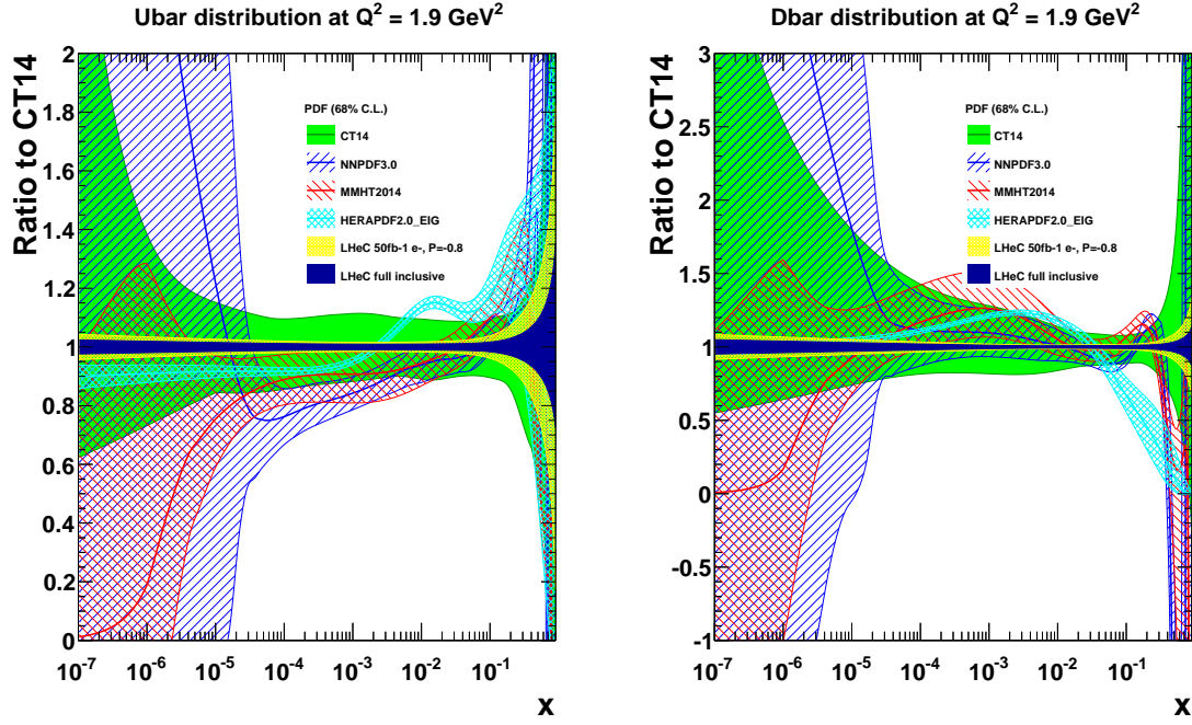
Figure 3.12: Sea quark distributions at Q^2 = 1.9 \text{ GeV}^2 as a function of Bjorken x , presented as the ratio to the CT14 central values. The yellow band corresponds to the LHeC 1st run PDFs ( D2 ), while the dark blue shows the LHeC full inclusive PDFs ( D4+D5+D7+D8 ), as described in the text. Both LHeC PDFs shown are scaled to the central value of CT14.
