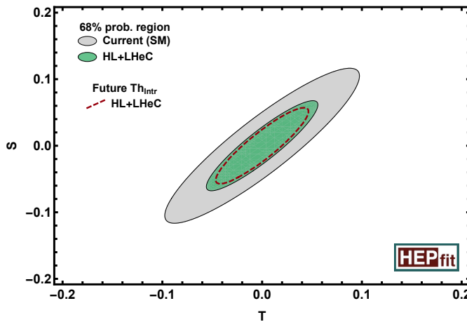
Figure 7.4: Allowed regions in the (S, T) plane. The grey and green areas indicate the currently allowed region and the LHeC projection, respectively. The dashed line indicates the effect of expected theoretical improvements. The HEPFIT program [2] was used for this analysis.
