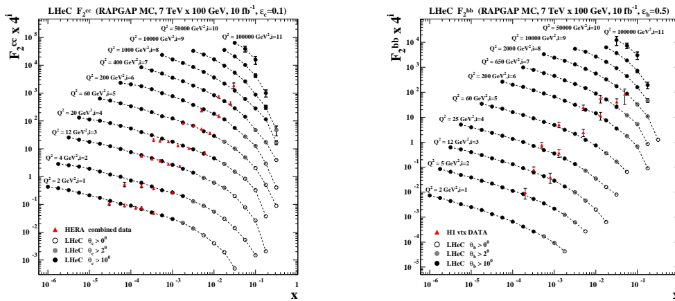
Figure 3.18: Heavy quark structure functions F_2^{c\bar{c}} and F_2^{b\bar{b}} showing the comparison of the HERA data to LHeC pseudodata.
