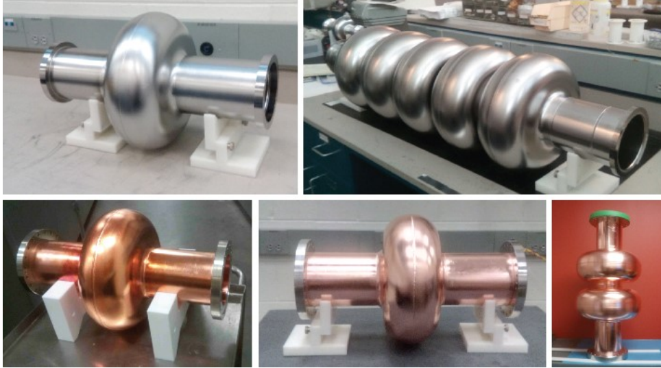
Figure 8.17: Ensemble of 802 MHz cavities designed and built at JLab for CERN. The Nb cavities have been tested vertically at 2 Kelvin in JLab’s vertical test area.
