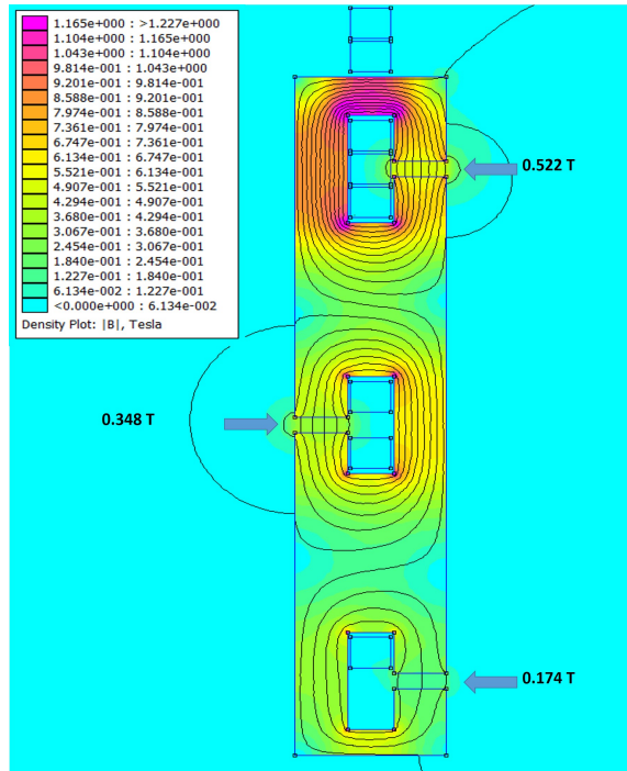
Figure 8.12: 50 GeV ERL - Cross section of the three apertures bending magnet, arc 2, 4 and 6 with 500 mm between neach arcs - FEM.
