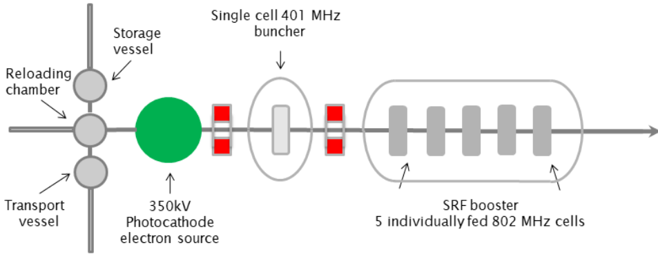
Figure 8.19: The layout of the unpolarised injector.
