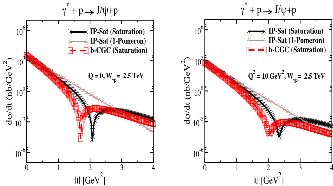
Figure 3.36: Differential cross section for elastic J/\psi production as a function of |t| within the IP-Sat (saturation), b-CGC and 1-Pomeron models at a fixed W\gamma p = 2.5 TeV, which corresponds to the region that can be explored by FCC-eh, and for two different values of photon virtuality Q = 0 (left plot) and Q^2 = 10 GeV 2 (right plot). The thickness of points includes the uncertainties associated with the freedom to choose different values for the charm quark mass within the range m_c = 1.2 - 1.4 GeV .
