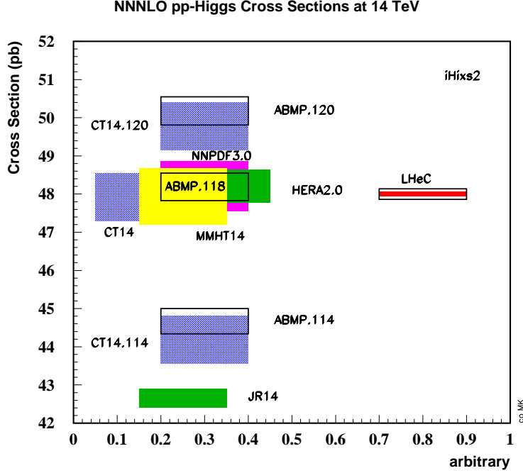
Figure 7.5: Cross sections of Higgs production calculated to N^3 LO using the iHix program [555] for existing PDF parameterisation sets (left side) and for the LHeC PDFs (right side). The widths of the areas correspond to the uncertainties as quoted by the various sets, having rescaled the CT14 uncertainties from 90 to 68% C.L. Results (left) are included also for different values of the strong coupling constant \alpha_s(M_Z^2) , from 0.114 to 0.120. The inner LHeC uncertainty band (red) includes the expected systematic uncertainty due to the PDFs while the outer box illustrates the expected uncertainty resulting from the determination of \alpha_s with the LHeC.
