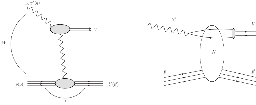
Figure 3.34: Left: diagram for the quasi-elastic production of the vector meson. Right: schematic illustration of the same process, quasi-elastic vector meson production, within the framework of the dipole picture. The initial virtual photon, fluctuates into a quark-antiquark pair which then scatters off the hadronic target and forms the vector meson. The details of the hadronic interaction of the dipole with the target are encoded in the dipole amplitude N .
