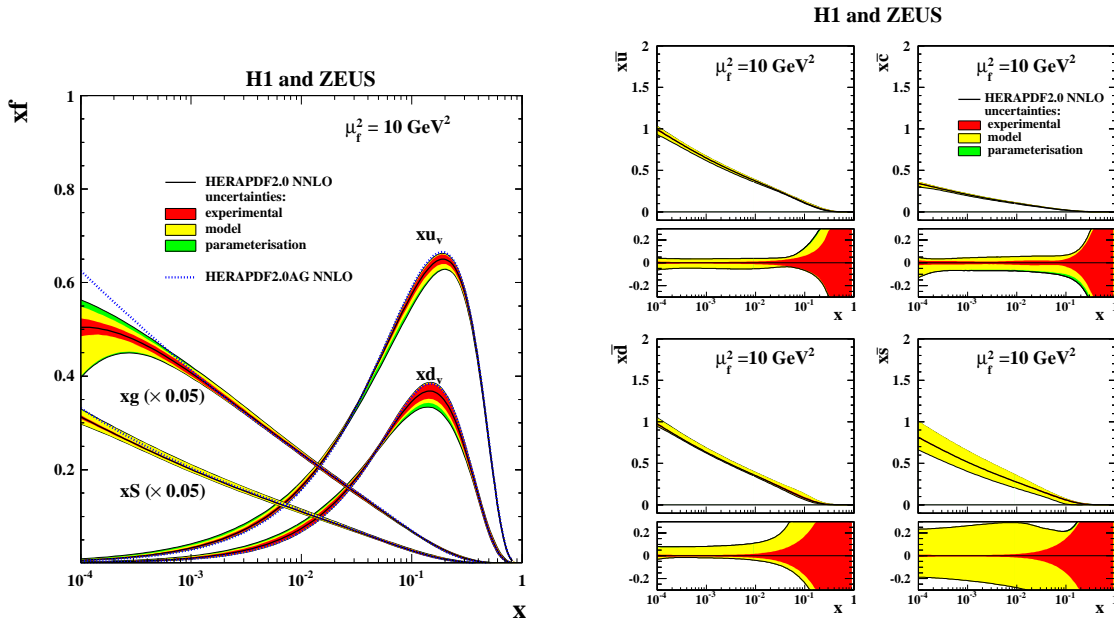
Figure 3.4: Left: HERAPDF2.0NNLO PDFs for valence, gluon and total Sea, showing experimental, model and parametrisation uncertainties separately, at factorisation scale \mu_f = 10 \text{ GeV}^2 . An alternative (AG) PDF with no negative term added to the gluon parametrisation is also shown. Right: HERAPDF2.0NNLO PDFs for the Sea, x\bar{u}, x\bar{d}, x\bar{c}, x\bar{s} showing experimental, model and parametrisation uncertainties separately, at factorisation scale \mu_f = 10 \text{ GeV}^2 . Fractional uncertainties are shown below the plots.
