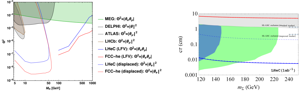
Figure 6.5: Left: Sensitivity of the LFV lepton-trijet searches (at 95 % C.L.) and the displaced vertex searches (at 95 % C.L.) from Ref. [506] compared to the current exclusion limits from ATLAS [508], LHCb [509], LEP [510], and MEG [511]. Right: Prospects of displaced vertex searches from charged fermion triplet \Sigma^\pm . The blue and green shaded regions denote the expected observability of 10 (100) events, dashed lines denote HL-LHC exclusion sensitivity, and the red line is connected to the light neutrino properties. For details, see text and Ref. [512].
