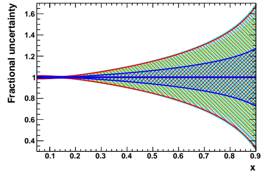
(b) Gluon distribution (linear x scale).
