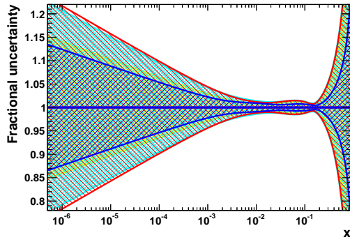
(a) Gluon distribution ( \log_{10} x scale)
