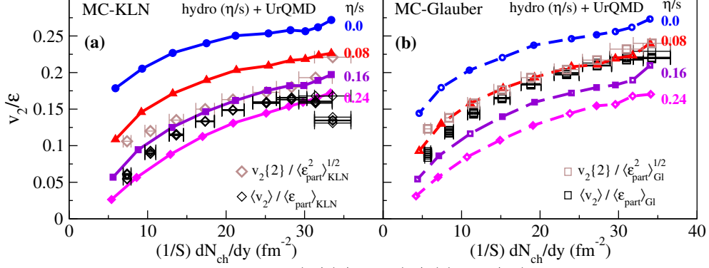
Figure 7.9: Comparison of the universal v_2(\eta/s)/\epsilon vs. (1/S)(dN_{\text{ch}}/dy) curves with experimental data for \langle v_2 \rangle [575], v_2\{2\} [576], and dN_{\text{ch}}/dy [577] from the STAR Collaboration. The experimental data used in (a) and (b) are identical, but the normalisation factors \langle \epsilon_{\text{part}} \rangle and S used on the vertical and horizontal axes, as well as the factor \langle \epsilon_{\text{part}}^2 \rangle^{1/2} used to normalize the v_2\{2\} data, are taken from the MC-KLN model in (a) and from the MC-Glauber model in (b). Theoretical curves are from simulations with MC-KLN initial conditions in (a) and with MC-Glauber initial conditions in (b). Taken from [571].
