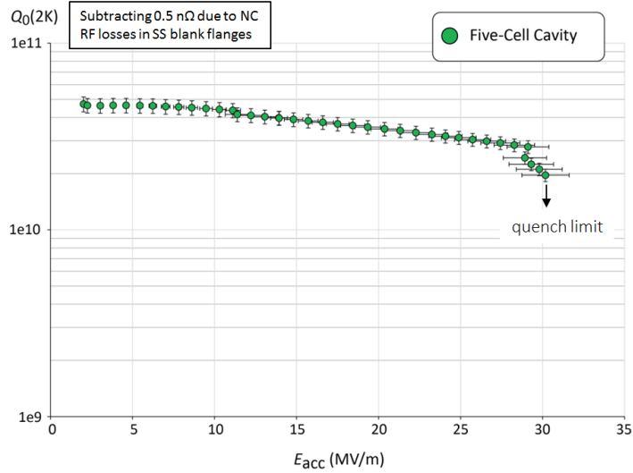
Figure 8.18: Vertical test result of the five-cell 802 MHz niobium cavity prototype.
