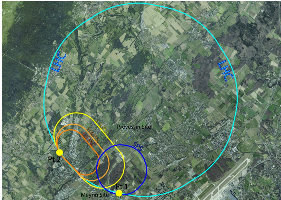
Figure 8.46: Racetrack options proposed for LHeC at Point 2 LHC. The color coding illustrated different options with 1/3 , 1/4 and 1/5 of the LHC circumference, resulting in different electron beam energies.
