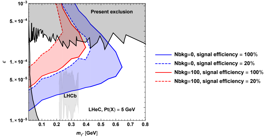
Figure 6.6: Projected sensitivity of dark photon searches at the LHeC via displaced dark photon decays from Ref. [519]. The sensitivity contour lines are at the 90 % confidence level and consider a transverse momentum cut on the final state hadrons of 5 GeV. The blue and red areas denote the assumption of zero and 100 background events, respectively, the solid and dashed lines correspond to a reconstruction efficiency of 100 % and 20 %, respectively. See Ref. [519] for details.
