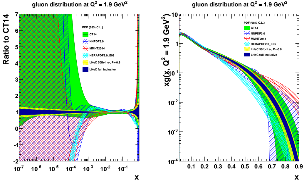
Figure 3.13: Gluon distribution at Q^2 = 1.9 \text{ GeV}^2 as a function of Bjorken x , highlighting (left) the low x and (right) the high x regions. The yellow band corresponds to the LHeC 1st Run PDFs ( D2 ), while the dark blue shows the LHeC full inclusive PDFs ( D4+D5+D7+D8 ), as described in the text. Both LHeC PDFs shown are scaled to the central value of CT14.
