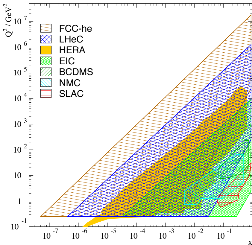
Figure 1.1: Coverage of the kinematic plane in DIS by some initial fixed target experiments with electrons (SLAC) and muons (NMS,BCDMS), by the future electron ion collider (EIC,green), HERA (yellow), the LHeC (blue) and the FCC-eh (brown). The low Q^2 region for the colliders is here limited to about 0.2 \text{ GeV}^2 , which is covered by the central detectors, roughly and perhaps using low electron beam data. Electron taggers may extend this to even lower Q^2 . The high Q^2 limit is given by the line of inelasticity y = 1 . Approximate limitations of acceptance at medium x , low Q^2 are drawn using polar angle limits of \eta = -\ln \tan \theta/2 of 4, 5, 6 for the EIC, LHeC, and FCC-eh, respectively. Since these lines are given by x = \exp \eta \cdot \sqrt{Q^2}/2E_p , it is clear that largest x values at low Q^2 are covered by the EIC (green area bottom, right).
