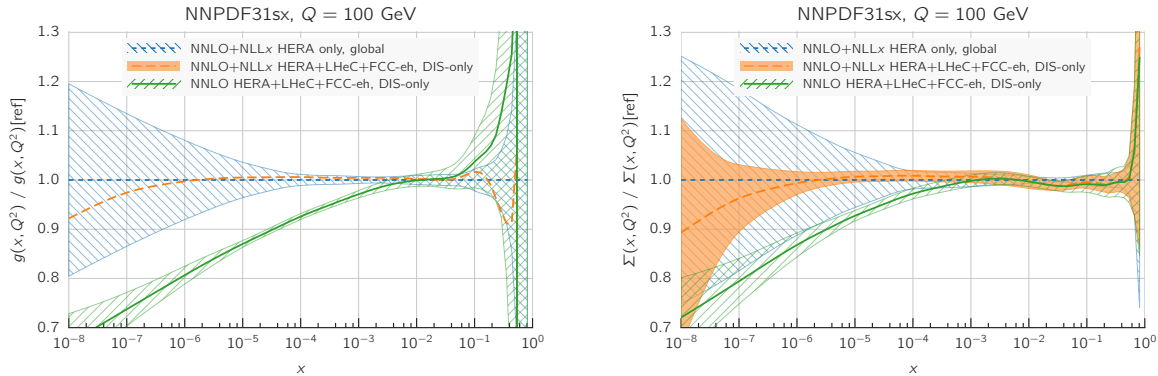
Figure 3.27: Comparison between the gluon (left plot) and the quark singlet (right plot) PDFs in the NNPDF3.1sx NNLO+NNLx fits without (blue hatched band) and with the LHeC+FCC-eh pseudodata (orange band) on inclusive structure functions. For completeness, we also show the results of the corresponding NNPDF3.1sx NNLO fit with LHeC+FCC-eh pseudodata (green hatched band). Figure taken from Ref. [190].
