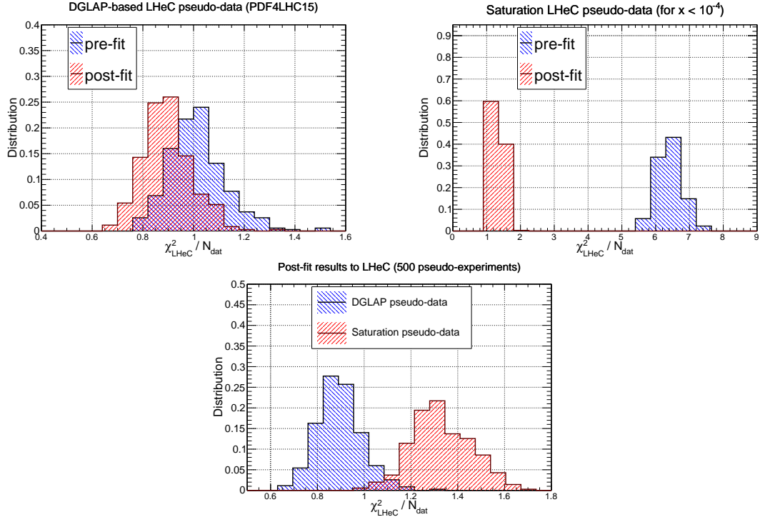
Figure 3.47: Upper plots: the distribution of pre-fit and post-fit values of \chi^2/n_{\text{dat}} for the N_{\text{exp}} = 500 sets of generated LHeC pseudodata. We compare the results of the profiling of the LHeC pseudodata based on DGLAP calculations in the entire range of x (left) with those where the pseudodata is based on the saturation model in the region x < 10^{-4} (right plot). Bottom plot: comparison of the post-fit \chi^2/n_{\text{dat}} distributions between these two scenarios for the pseudodata generation.
