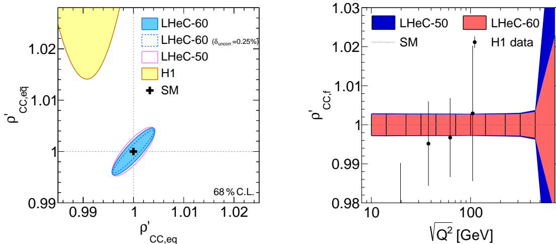
Figure 3.57: Left: anomalous modifications of the charged current form factors \rho'_{CC,eq} and \rho'_{CC,e\bar{q}} for different LHeC scenarios in comparison with the H1 measurement [316]. Right: scale dependent measurement of the anomalous modification of the charged current form factor \rho'_{CC}(Q^2) , assuming \rho'_{CC,eq} = \rho'_{CC,e\bar{q}} = \rho'_{CC} .
