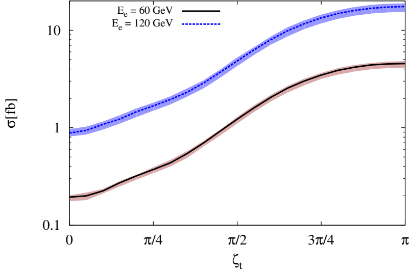
Figure 5.4: Total cross section of the Higgs boson produced in association with a single top as a function of \zeta_t , including scale uncertainties. The black solid and blue dotted lines correspond to E_e = 60 and 120 GeV, respectively. These are obtained for fixed E_p = 7 TeV and scales \mu_F = \mu_R = (m_t + m_h)/4 .
