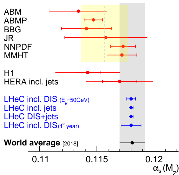
Figure 3.25: Summary of \alpha_s(M_Z) values in comparison with present values.
