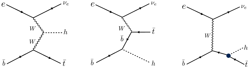
Figure 5.2: Leading order Feynman diagrams contributing to the process p e^- \rightarrow \bar{t} h \nu_e in high energy e^- p collisions. The black dot in the Feynman diagram on the right denotes the top-quark-Higgs coupling of interest in this section.
