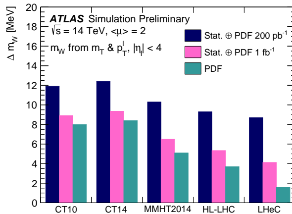
Figure 7.2: Measurement uncertainty for different PDF sets, combining p_T^\ell and m_T fits for |\eta| < 4 , and for 200 \text{ pb}^{-1} and 1 \text{ fb}^{-1} collected at \sqrt{s} = 14 \text{ TeV} .
