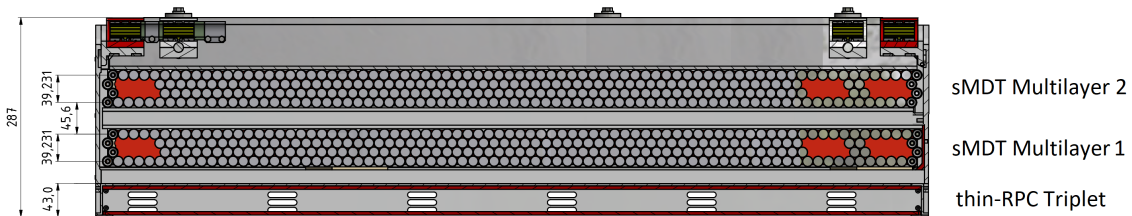
Figure 10.11: A transverse view of a RPC-MDT assembly as adapted from a drawing of the ATLAS Phase 1 muon upgrade [?]. In this case a station is composed of an RPC triplet for trigger and 2-coordinate readout and two MDT superlayers for precise track measurements.
