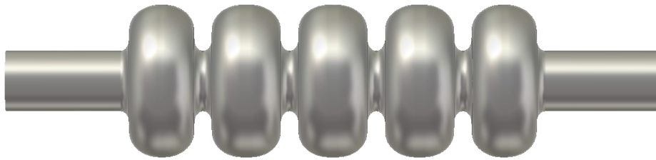
Figure 8.15: Bare 802 MHz five-cell cavity design (RF vacuum) with a 130 mm iris and beam tube aperture.
