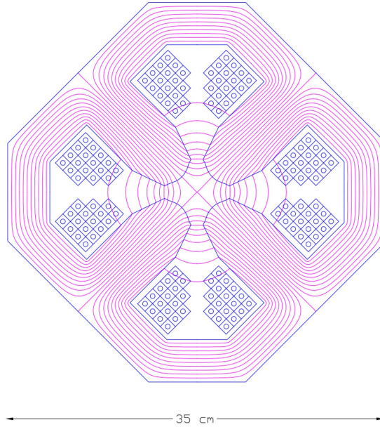
Figure 8.13: 50 GeV ERL - Cross section of the arc quadrupole magnets.
