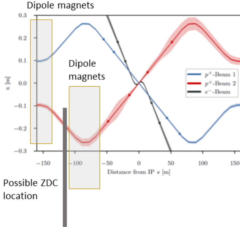
Figure 10.12: Possible location of a ZDC for the linac–ring design of LHeC. The solid rectangle represents the ZDC. The two boxes in front of and behind the ZDC indicate the locations for bending magnets.
