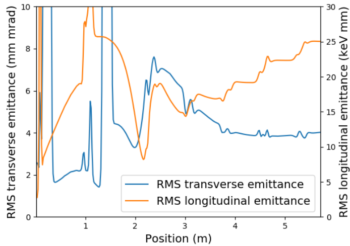
Figure 8.22: The emittances of the bunch as it travels along the injector.
