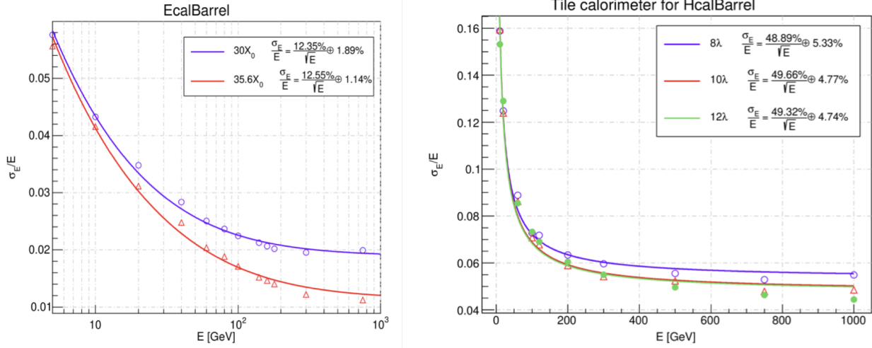
Figure 10.9: Crystal Ball fitted energy dependent resolution for the barrel electromagnetic (left) and barrel hadronic (right) calorimeters EMC and HCAL, respectively. The first ( a ) term includes shower fluctuations and transverse leakages and the second ( b ) term includes leakages from the calorimeter volume longitudinally.
