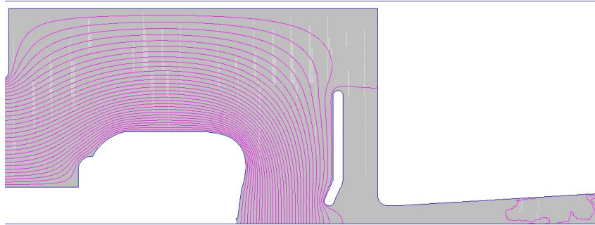
Figure 8.20: The optimised electrode geometry for PERLE. This is a Jefferson lab type gun and is optimised for both 350 kV and 220 kV operation.
