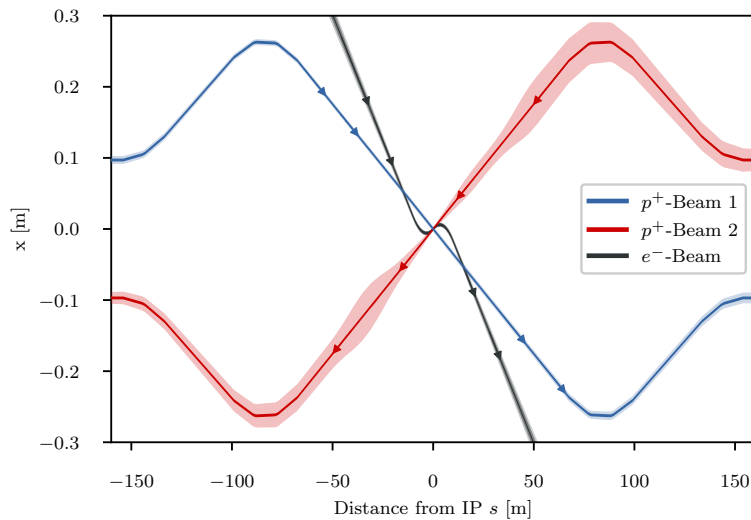
Figure 8.25: Geometry of the interaction region with 10\sigma envelopes. The electron beam is colliding with the focussed anti-clockwise rotating LHC beam (Beam 2) while the clockwise rotating LHC beam is unfocussed and passes the Interaction Region without interacting with the other two beams
