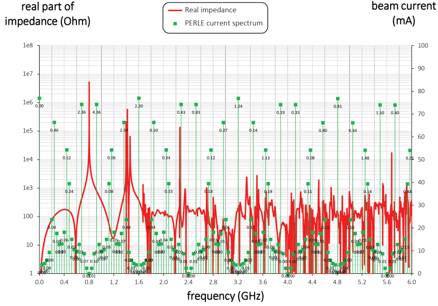
Figure 8.16: Real monopole impedance spectrum of the five-cell 802 MHz cavity prototype (red) together with the considered beam current lines (green) for the 3-pass PERLE machine (25 mA injected current). The numbers associated with the spectral lines denote the power dissipation (in Watt).
