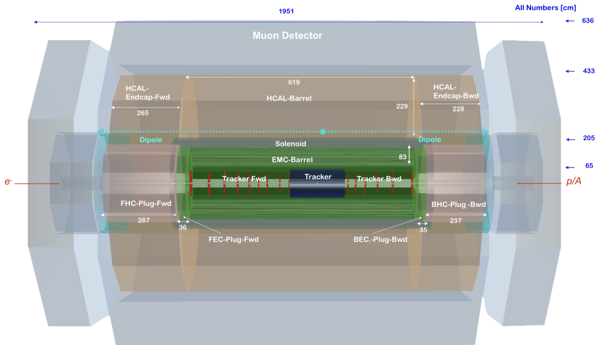
Figure 10.13: Side view of a low energy FCCeh ( E_p = 20\text{TeV} ) concept detector, designed using the DD4hep framework [668], showing the essential features. The solenoid is again placed between the ECAL-Barrel and Hadronic-Barrel calorimeters and is housed in a cryostat in common with the beam steering dipoles extending over the full length of the barrel and plug hadronic calorimeters. The sizes have been chosen such that the solenoid/dipoles and ECAL-Barrel systems as well as the whole tracker are also suitable to operate after an upgrade of the beam energy to E_p = 50\text{TeV} .
