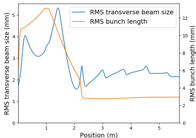
Figure 8.21: The rms beam sizes transversely and longitudinally as the bunch travels along the injector.
