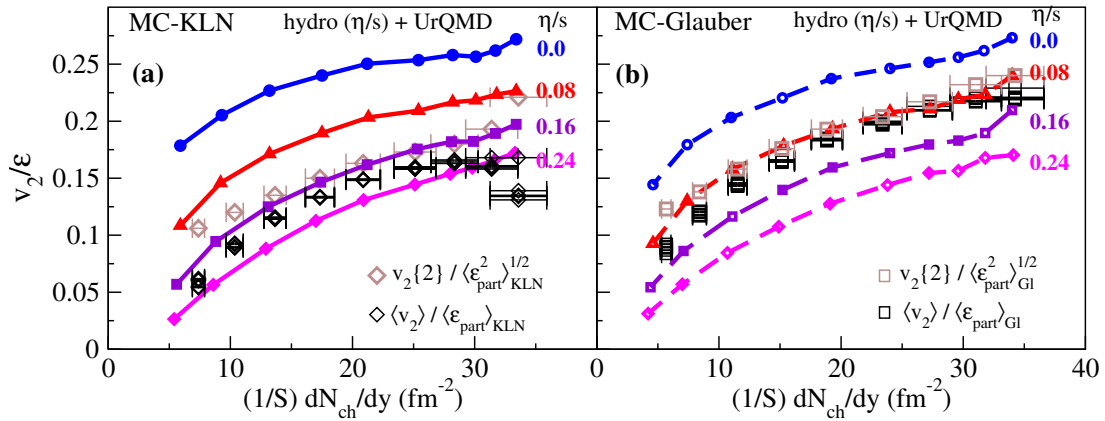
Figure 9.16: Comparison of the universal v_2(\eta/s)/\epsilon vs. (1/S)(dN_{\text{ch}}/dy) curves with experimental data for \langle v_2 \rangle [775], v_2\{2\} [776], and dN_{\text{ch}}/dy [777] from the STAR Collaboration. The experimental data used in (a) and (b) are identical, but the normalisation factors \langle \epsilon_{\text{part}} \rangle and S used on the vertical and horizontal axes, as well as the factor \langle \epsilon_{\text{part}}^2 \rangle^{1/2} used to normalize the v_2\{2\} data, are taken from the MC-KLN model in (a) and from the MC-Glauber model in (b). Theoretical curves are from simulations with MC-KLN initial conditions in (a) and with MC-Glauber initial conditions in (b). Taken from [771].
