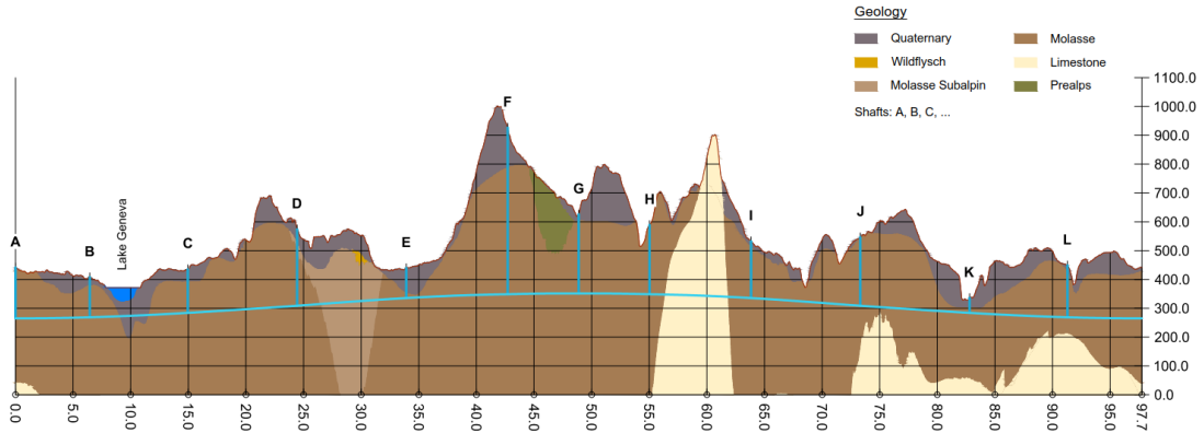
Figure 10.56: Geological profile along FCC tunnel circumference
