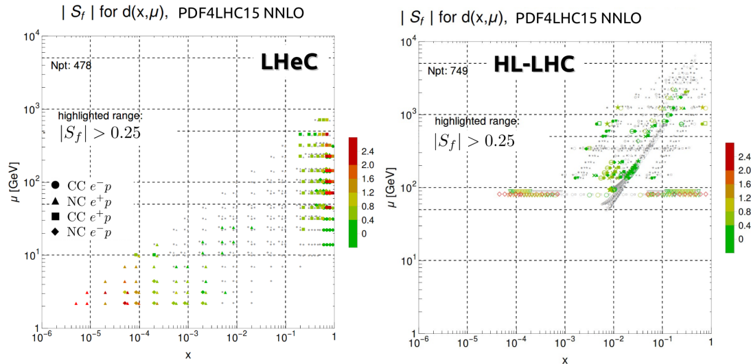
Figure 9.11: Sensitivity for a sample flavour \{d(x, Q)\} in the \{x, Q^2\} kinematic plane for the LHeC (left) and the HL-LHC (right) calculated with pseudodata [746]. We observe the LHeC is particularly sensitive in both the high and low x regions, and the HL-LHC covers the intermediate x region out to large Q scales.
