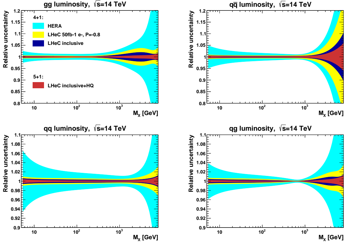
Figure 3.21: Uncertainty bands for parton luminosities as a function of the mass M_X = \sqrt{sx_1x_2} for LHC energies. Light blue: fit to HERA data using the same parameterisation as the LHeC fits shown; yellow: expectation from the first run period of the LHeC with solely e^-p operation; dark blue: inclusive fit, based on the data sets (D4+D5+D6+D9) in Tab. 3.2; red: fit to the inclusive data adding simulated heavy flavour s , c , b data with a 5 quark distribution parameterisation as introduced above.
