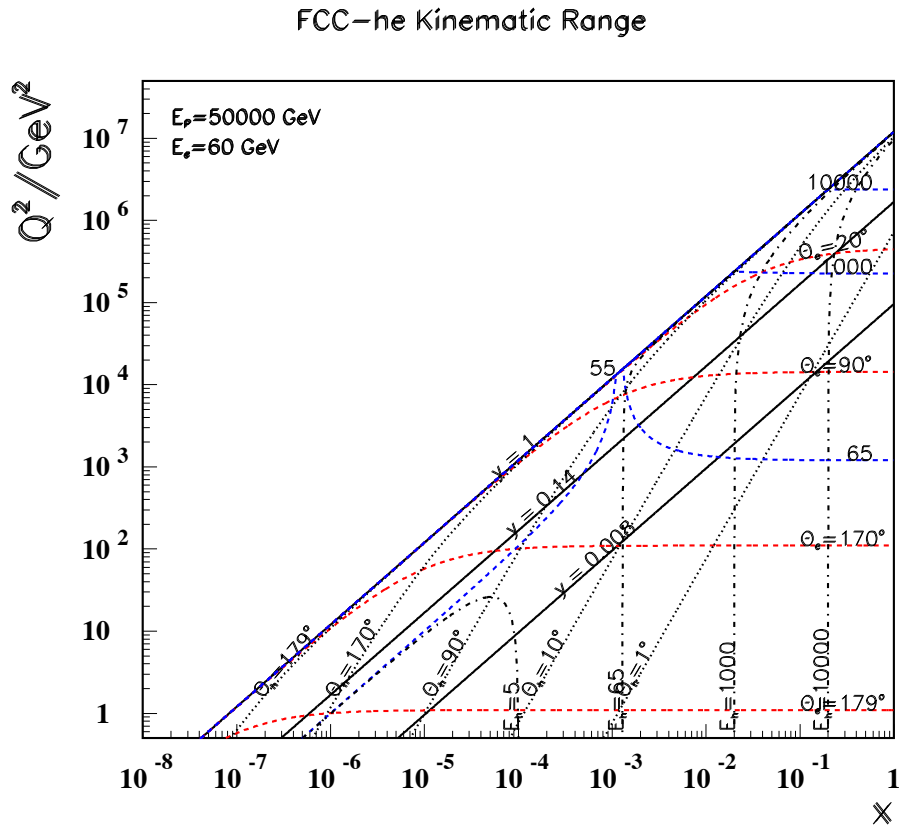
Figure 5: Kinematics of the FCC-he for E_p = 50 TeV and E_e = 60 GeV. Blue dashed: lines of constant scattered electron energy, which for Q^2 below 1000 GeV 2 never exceeds 65 GeV. Red dashed: lines of constant electron polar angle. One observes that the low x region is very well accessible with a detector acceptance to backward electrons down to one degree. Black dashed-dotted: lines of constant hadronic final state energy. At large Borken x , energies of up to tens of TeV are scattered in the forward detector region; Black dotted: lines of constant polar angle of the hadronic final state. One can see that the high x , medium Q^2 \sim 10^{3-4} GeV 2 region is hardly accessible with the FCC-he, it yet would have been covered by the LHeC before.
