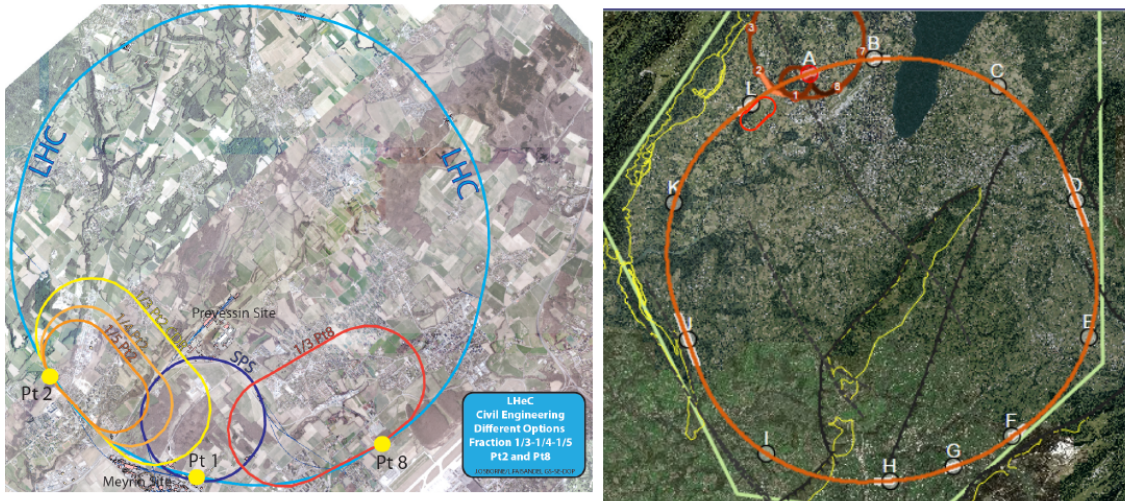
Figure 2: Possible locations of the ERL racetrack electron accelerator for the LHeC (left) and the FCC-he (right). The LHeC is shown to be tangential to Point 2 and Point 8. For Point 2 three sizes are drawn corresponding to a fraction of the LHC circumference of 1/3 (outer, default with E_e = 60 GeV), 1/4 (the size of the SPS, E_e = 56 GeV) and 1/5 (most inner track, E_e = 52 GeV). To the right one sees that the 8.9km default racetrack configuration appears to be rather small as compared to the 100 km ring of the FCC. Present considerations suggest that Point L may be preferred as the position of the ERL, while two GPDs would be located at A and G.
