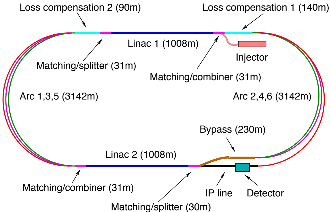
Figure 3: Schematic view of the default LHeC configuration. Each linac accelerates the beam to 10 GeV, which leads to a 60 GeV electron energy at the interaction point after three passes through the opposite lying linac structures made of 60 cavity-cryo modules each. The arc radius is about 1 km and the circumference chosen to be 1/3 of that of the LHC. The beam is decelerated for recovering the beam power after having passed the IP.
