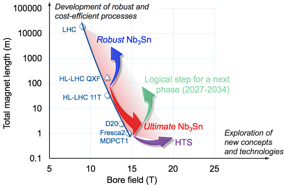
Fig. 2.7: Graphical representation of the objective of the HFM R&D programme in this phase, 2021–2027. Both fronts of maximum field (red for Nb 3 Sn, purple for HTS) and large-scale production (blue) are intended to be advanced at the same time. Also represented, in green, is a possible evolution for the longer term, 2027–2034.
