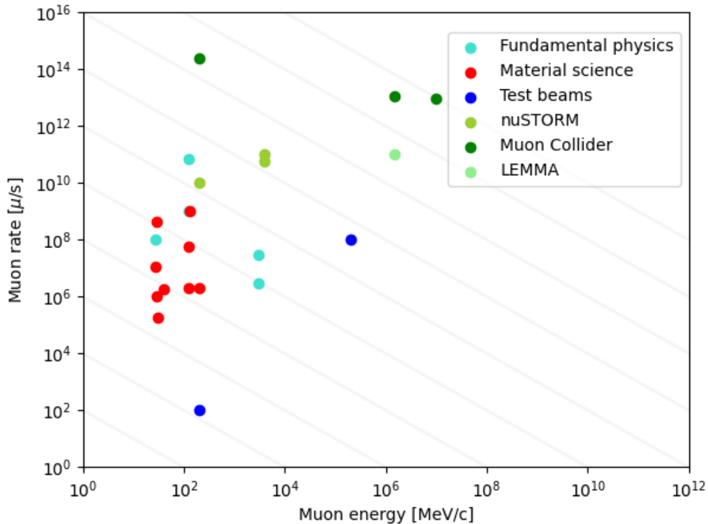
Fig. 4.10: Existing and proposed muon sources as a function of muon rate and muon energy. Diagonal lines show contours of equal beam power. Where available, muon rate data is taken near to the target. For muon collider and nuSTORM, multiple values are shown corresponding to different design options and regions of the facility.
