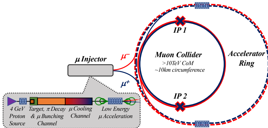
Fig. 4.1: A conceptual scheme of the muon collider.
