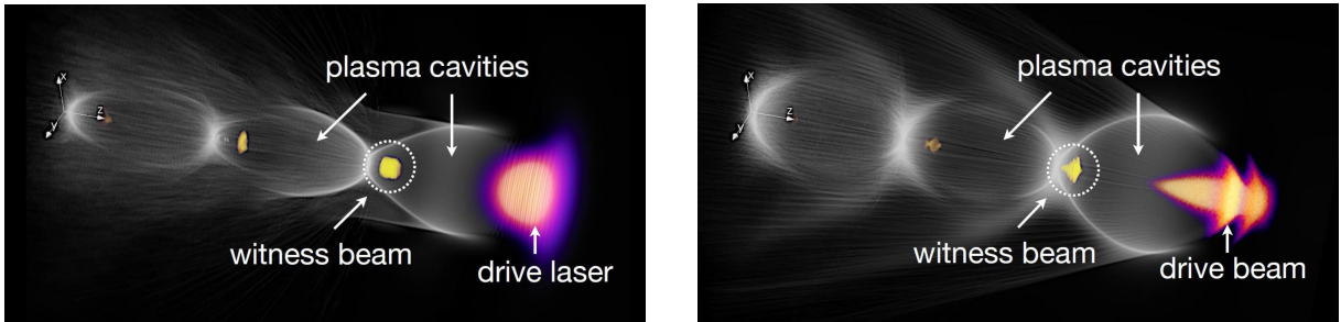
Fig. 3.9: Simulation of a LWFA ( left ) and a PWFA ( right ), showing the formation of the accelerating cavities in the plasma. The witness beam is located at the point where the accelerating field is highest, just before the end of the first bubble. Image credit: EuPRAXIA Conceptual Design Report, A. Martinez de la Ossa
