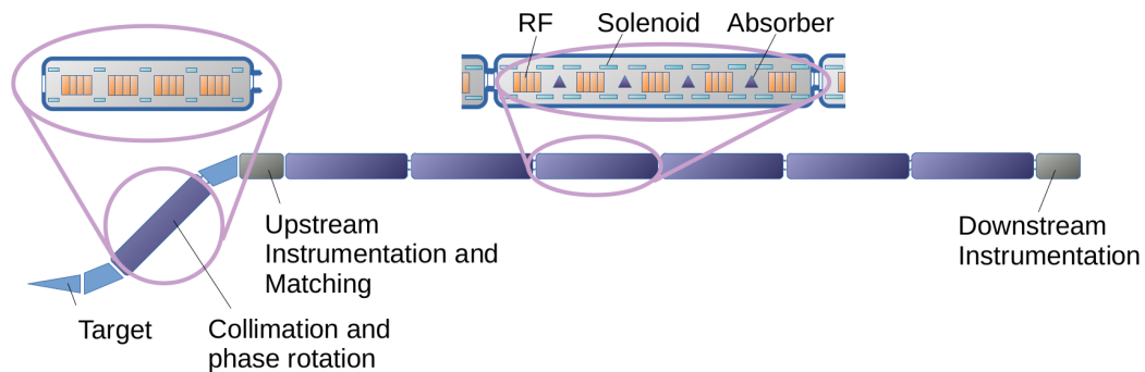
Fig. 4.11: Schematic diagram of a possible implementation of the muon cooling demonstrator. A pion-production target is followed by a collimation and phase rotation section where a low emittance muon beam is created. Instrumentation upstream and downstream of the cooling region is used to determine muon beam properties before and after a number of ionisation cooling cryostats, each containing a series of solenoids and RF cavities.
