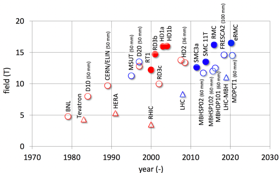
Fig. 2.1: Fields attained with Nb 3 Sn dipole magnets of various configurations and dimensions and either at liquid (4.2 K, red) or superfluid (1.9 K, blue) helium temperature. Solid symbols are short demonstrator, i.e. “racetracks” with no bore, while open symbols are short models and long magnets with bore. For comparison, superconducting collider dipole magnets past and present are shown as triangles.
