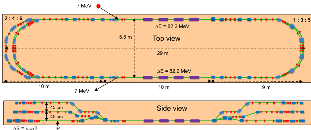
Fig. 5.3: Top and side views of the PERLE facility at IJCLab Orsay. An electron energy of 500 MeV is achieved in three turns passing through two cryomodules, each housing four 5-cell cavities of 802 MHz frequency. PERLE will be built in two stages, first with one linac cryomodule, adapted from the SPL module, and then completed with a newly designed one. The total number of magnets, including arcs, switchyards, merger and experiments, is 84 dipoles, 33 or 66 cm long, of typically 0.5–1 T bend and 118 quadrupoles, 10 to 15 cm long, with fields between 0.4 and 5.5 kG/cm. Optics and further features of this configuration are briefly discussed below.
