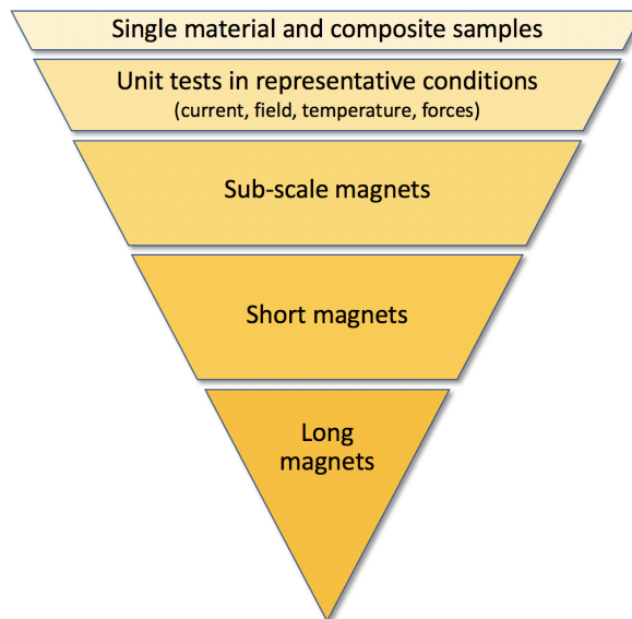
Fig. 2.10: Schematic representation of the innovation funnel concept, conducive to fast turnaround technology development.
