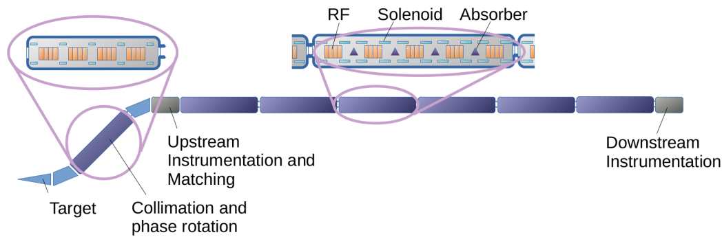
Fig. 5.11: Schematic diagram of a possible implementation of the muon cooling demonstrator. A pion-production target is followed by a collimation and phase rotation section where a low emittance muon beam is created. Instrumentation upstream and downstream of the cooling region is used to determine muon beam properties before and after a number of ionisation cooling cryostats, each containing a series of solenoids and RF cavities.
