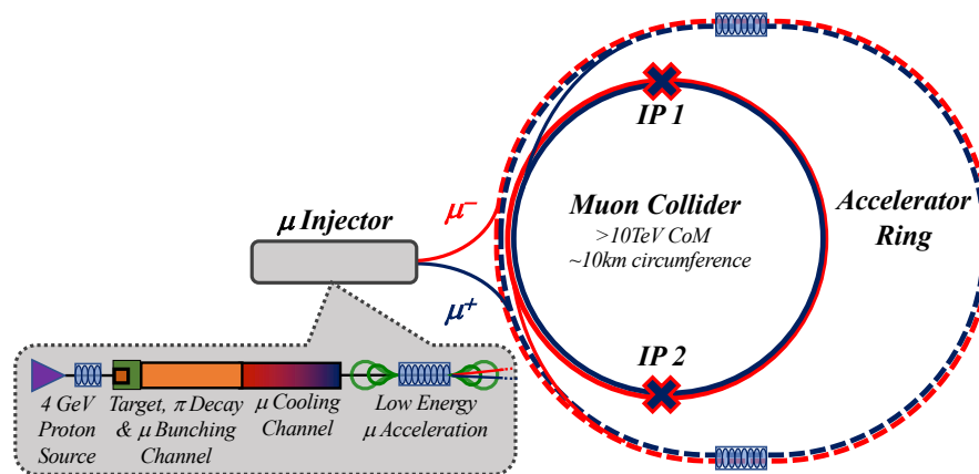
Fig. 5.1: A conceptual scheme for the muon collider.
