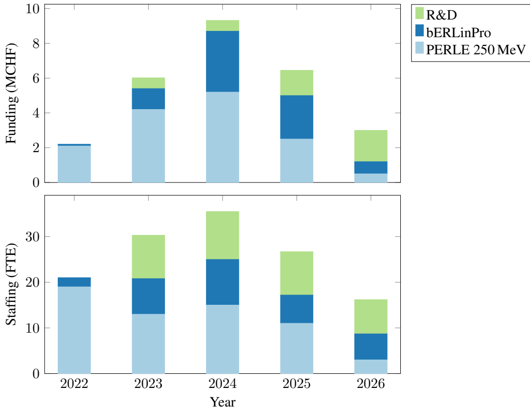
Fig. 6.11: ERL funding and effort roadmap profile for the next five years, split into its three main contributions, PERLE at 250 MeV, bERLinPro and the key R&D items (HOM, TWN and DIA): top: annual spending in MCHF; bottom: effort in FTE years, not counting provision of effort by the host laboratories and some of their partners.
