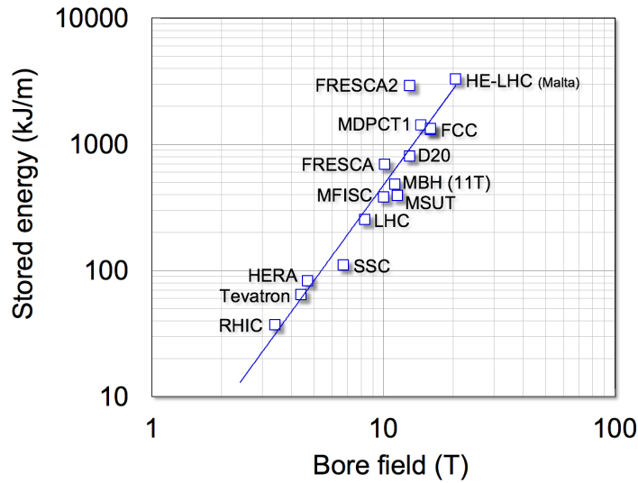
Fig. 2.5: Scaling of stored energy per unit length for dipole magnets built or designed (values refer to one aperture in case of the LHC, 11T, FCC and HE-LHC). The line is proportional to B^{2.5}
