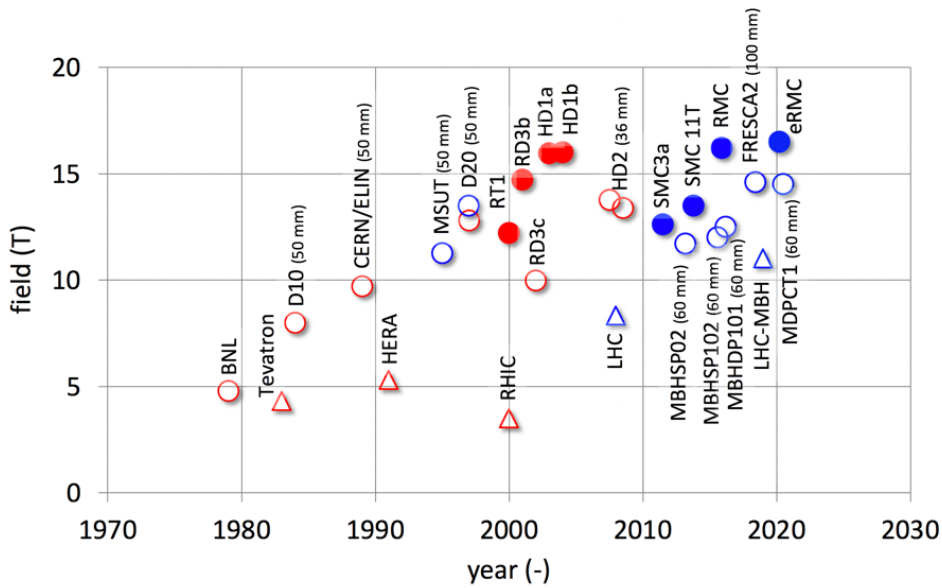
Fig. 2.1: Fields attained with Nb 3 Sn dipole magnets of various configurations and dimensions, either at liquid (4.2 K, red) or superfluid (1.9 K, blue) helium temperature. Solid symbols are short demonstrators, i.e. ‘racetracks’ with no bore, while open symbols are short models and long magnets with bore. For comparison, superconducting collider dipole magnets past and present are shown as triangles.
